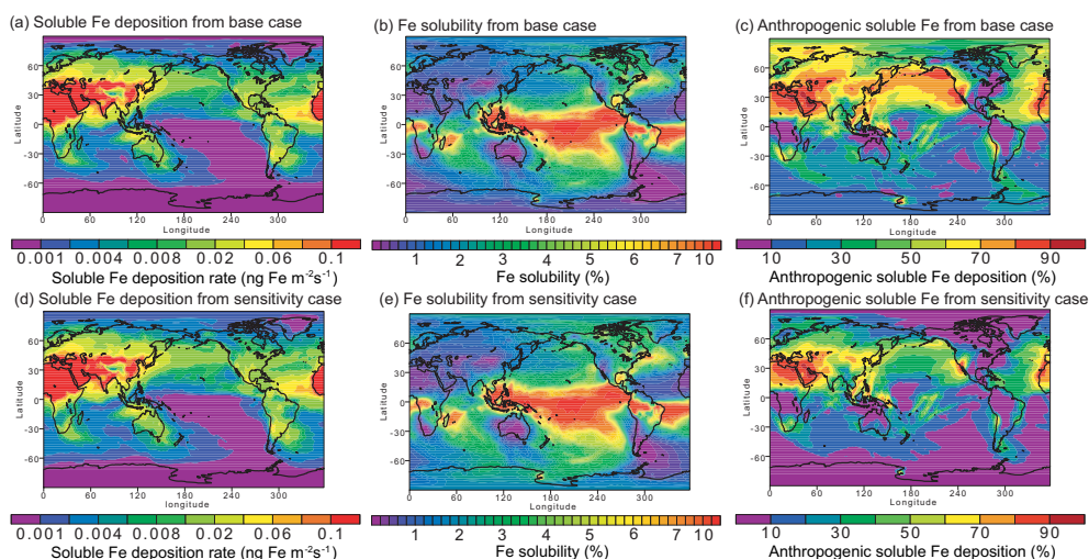
Figure 7. Deposition of soluble Fe ( \text{ng Fe m}^{-2}\text{s}^{-1} ) from dust and combustion sources to the oceans in the present day (a) from base simulations and (d) from sensitivity simulations, Fe solubility in the present day (b) from base simulations and (e) from sensitivity simulations, and ratio of increase from the preindustrial era to present day to soluble Fe deposition in the present day (c) from base simulations and (f) from sensitivity simulations. The formation of the amorphous \text{Fe}(\text{OH})_3(\text{s}) suppresses the oxalate-promoted dissolution from mineral aerosols in the base simulations, while no such effect was considered for quasi-light-induced reductive dissolution in the sensitivity simulation (i.e., f_3 = 1 ).
