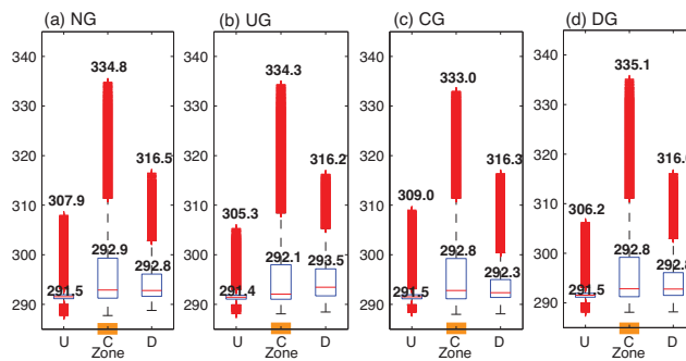
Figure 11. As in Fig. 8 but for temperature (K).
