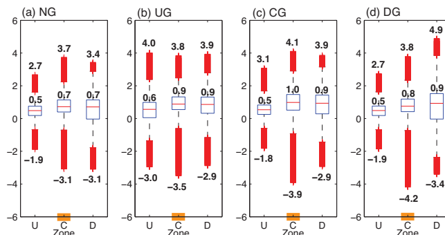
Figure 8. Box and whisker plots of instantaneous u component of the wind ( \text{m s}^{-1} ) within the canopy for case (a) NG, (b) UG, (c) CG, and (d) DG. From left to right in each panel, plots correspond to grid points in the upstream, center, and downstream zones (see Fig. 1 and canopy outlines in Fig. 2b–d for illustration of zones); fire location indicated by orange rectangle. For each box and whisker plot, the top and bottom of the box denotes the 75 % ( q_3 ) and 25 % ( q_1 ) percentiles, the horizontal red line denotes the median, the whiskers extend away from the box to the highest and lowest points not considered outliers, and the red bars extend outward from the whiskers to the maximum and minimum values. Note that the median, maximum, and minimum values are labeled for each plot.
