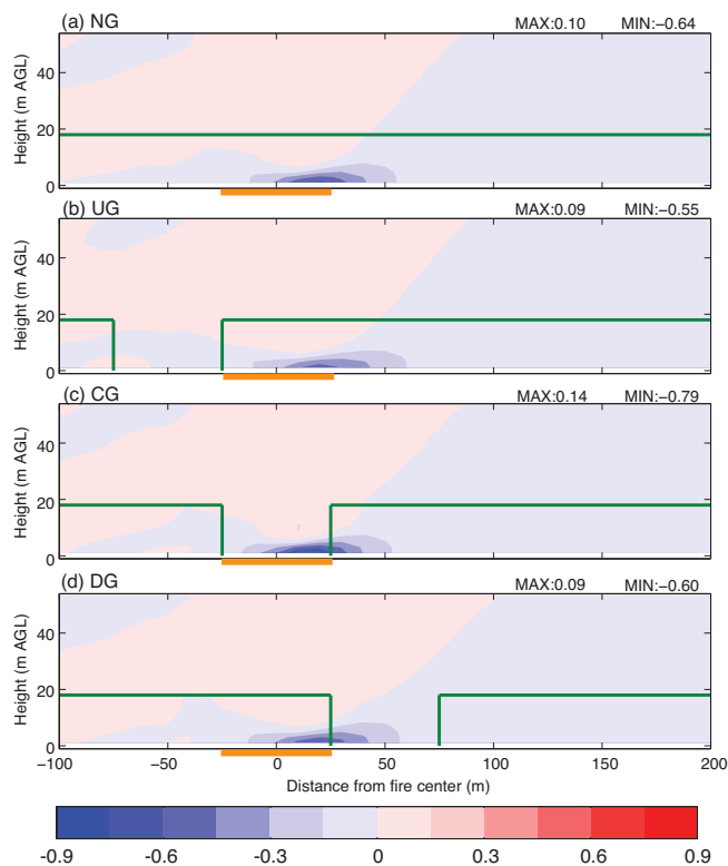
Figure 6. As in Fig. 2 but for the vertical gradient of the vertical turbulent heat flux ( \text{K s}^{-1} ); shading interval: 0.15 \text{ K s}^{-1} . The no-fire case is omitted due to small values relative to fire case.
