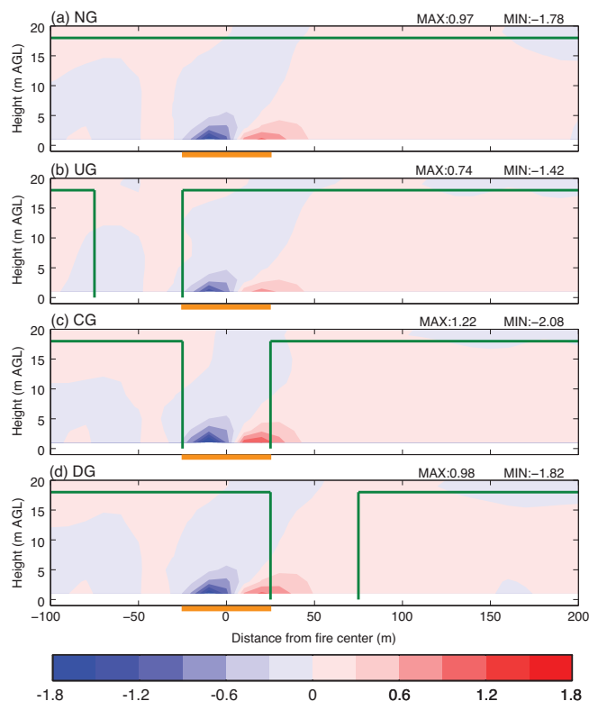
Figure 7. As in Fig. 2 but for the horizontal gradient of the horizontal turbulent heat flux ( \text{K s}^{-1} ); shading interval: 0.3 \text{ K s}^{-1} . Note that the y axis only extends up to 20 m a.g.l.
