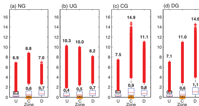
Figure 10. As in Fig. 8 but for TKE ( \text{m}^2 \text{ s}^{-2} ).
