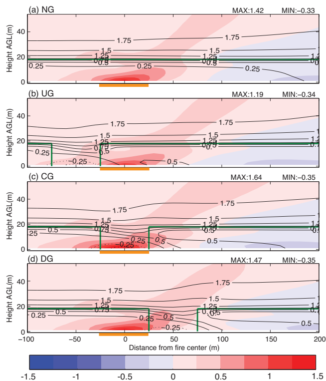
Figure 2. Vertical cross sections of the u component of the wind ( \text{m s}^{-1} ), averaged in time (30 min) and space (along fire line); contours denote the no-fire case ( 0.25 \text{ m s}^{-1} interval), and shading depicts the difference between the fire and no-fire cases ( 0.25 \text{ m s}^{-1} interval). The fire zone is denoted with an orange line, and the perimeter of the forest canopy is indicated with a green line. The maximum and minimum fire–no-fire difference for each case is included above each panel. Note that only a subset of the domain is displayed in each panel (100 m upstream to 200 m downstream of the fire center); see Fig. 1.
