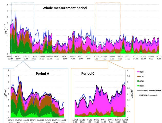
Figure 11. Time series of hourly averaged AMS ME-2 OOA factors, WSOC measured, and WSOC reconstructed for the whole measurement period (top), Period A (bottom left), and Period C (bottom right) at SPC. The units for each OOA factor have been converted from \mu\text{g m}^{-3} to \mu\text{g C m}^{-3} using their calculated OM / OC ratio.
