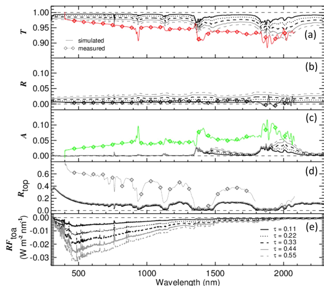
Figure 10. The lines show simulated, spectral (a) transmissivity, (b) reflectivity, and (c) absorptivity of a cirrus layer between 9 and 9.2 km altitude. Panel (e) shows the radiative forcings at TOA, respectively. The simulations are based on a measured number size distribution assuming the mixture of shapes according Baum et al. (2005). Inserted is the measurement case (diamonds) from Fig. 7.
