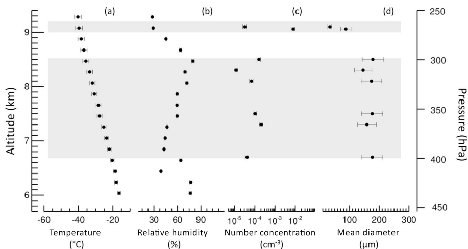
Figure 5. Vertical profiles of (a) temperature, (b) relative humidity, measured on the Learjet 35A, (c) number concentration, and (d) mean diameter, derived by CIPGs on AIRTOSS, from the flight of 30 August 2013. The bars show the corresponding measurement uncertainties. The gray areas indicate the vertical extent of the cirrus layers.
