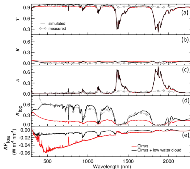
Figure 12. Same as Fig. 10 assuming the mixture according to Baum et al. (2005) between 6.7 and 8.5 km altitude ( \tau_{\text{Cirrus}} = 1 ). An additional low water cloud with \tau = 20 is included between 1.0 and 1.25 km altitude. Inserted is the measurement case (gray diamonds).
