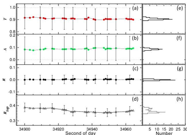
Figure 8. Time series of (a) transmissivity, (b) absorptivity, and (c) reflectivity (at 1640 nm) for the cirrus layer between 9.0 and 9.2 km altitude on 30 August 2013. The associated cloud top albedo is plotted in (d). The vertical bars represent the errors due to measurement uncertainties. Panels (e)–(h) show the histograms, respectively.
