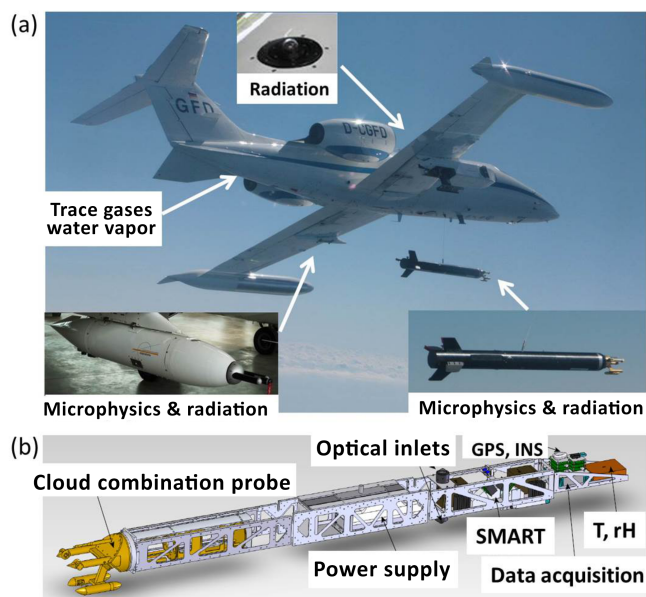
Figure 2. (a) Assembly of the research aircraft Learjet 35A, the towed AIRTOSS, and the wing pod containing instruments measuring radiation, microphysical parameter, water vapor, and trace gases. (b) Sketch of the AIRTOSS setup.
