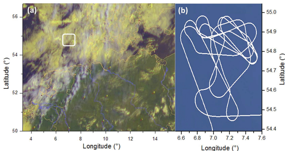
Figure 4. (a) Composite satellite image of the cloud situation on 30 August 2013 at 09:45 UTC showing high-level cirrus (white) above low-level water clouds (yellow, Deutscher Wetterdienst/EUMETSAT). In (b) the flight track of the measuring flight in the restricted area (white box in (a)) above the North Sea near the island of Helgoland, north Germany, is shown.
