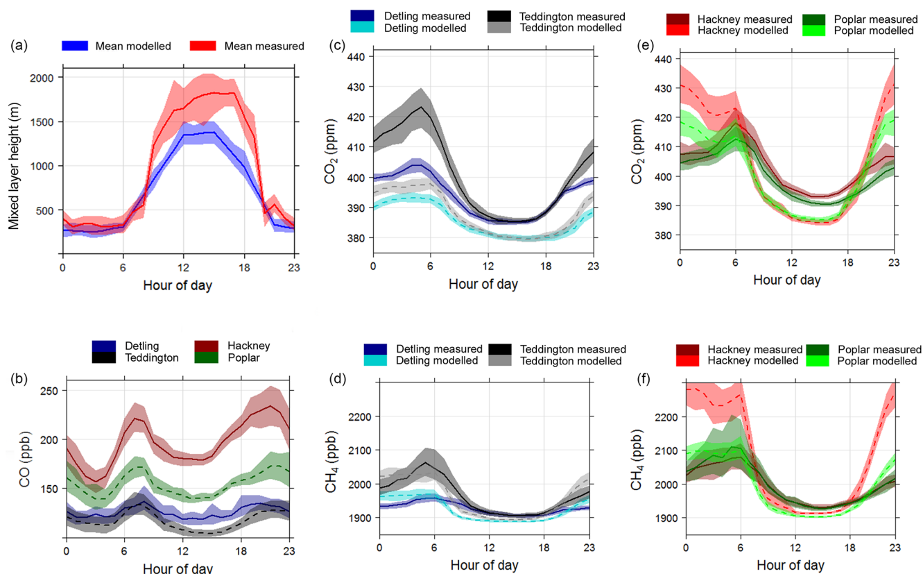
Figure 3. Mean diurnal cycles of (a) modelled (blue) and measured (red) boundary layer height and measured mean mixing layer height at North Kensington based on the spectral correction method described in Sect. 2.5, (b) measured CO mole fractions at the rural (Detling, blue), suburban (Teddington, black), and urban sites (Hackney, red; Poplar, green), (c) modelled (light shade) and measured (dark shade) CO 2 mole fractions at the rural (Detling, blue) and suburban (Teddington, black) sites, (d) modelled and measured (dark shade) CH 4 mole fractions at the rural (Detling, blue) and suburban (Teddington, black) sites, (e) modelled (light shade) and measured (dark shade) CO 2 mole fractions at the urban (Hackney, red; Poplar, green) sites and (f) modelled and measured CH 4 mole fractions at the urban (Hackney, red; Poplar, green) sites. June data are excluded due to unavailability of data during this period at Detling. Shading represents an estimate of the 95 % confidence interval in the mean, related to the limitation of the sampling of the daily values at a given hour, assuming these values are independent (based on the division of 2 times their temporal standard deviation by the square root of the number of values).
