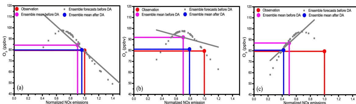
Figure 4. (a–c) O 3 concentrations (ppbv) and NO x emissions (no unit, normalized by the true NO x emission) before and after data assimilation and their ensemble samples before DA at 12:00 LT on 12 August 2008 in the three ideal ozone data assimilation experiments with the prior NO x emissions underestimated by 10 % (a), 30 % (b), and 50 % (c), respectively. The grey squares denote the ensemble forecast O 3 concentrations corresponding to the perturbations of the NO x emissions (ensemble forecasts before DA), and the magenta dot represents the result of the ensemble mean of the grey squares (ensemble mean before DA). The gray line represents a linear relationship calculated from the ensemble samples of O 3 concentrations and NO x emissions. The red dot represents the true state of the NO x emission and the observed O 3 concentration. The analyzed O 3 concentration and NO x emission are denoted by the blue dot.
