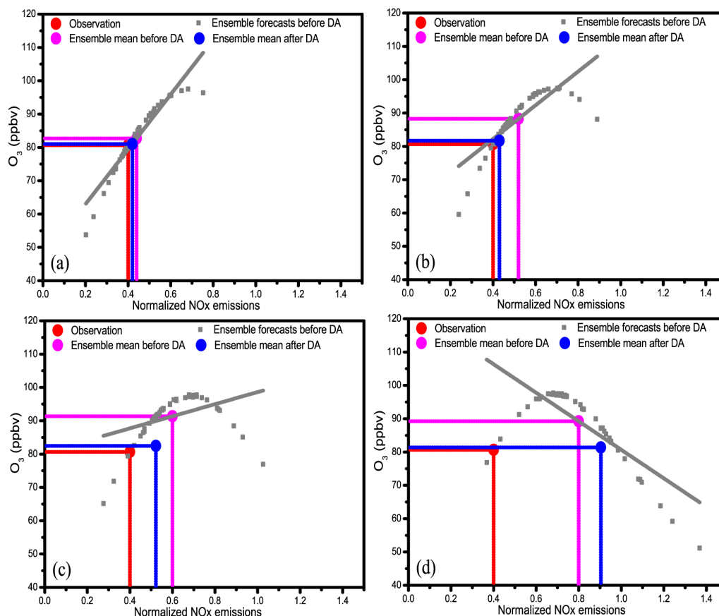
Figure 5. (a–d) O 3 concentrations (ppbv) and NO x emissions (no unit, normalized by the true NO x emission) before and after data assimilation and their ensemble samples before DA at 12:00 LT on 12 August 2008 in the four idealized DA experiments. (a) DA experiment with 10 % overestimate in the a priori NO x emission; (b) DA experiment with 30 % overestimate in the a priori NO x emission; (c) DA experiment with 50 % overestimate in the a priori NO x emission; (d) DA experiment with 100 % overestimate in the a priori NO x emission. The magenta dot, the gray squares, the gray line, the red dot, and the blue dot represent the same information as in Fig. 4.
