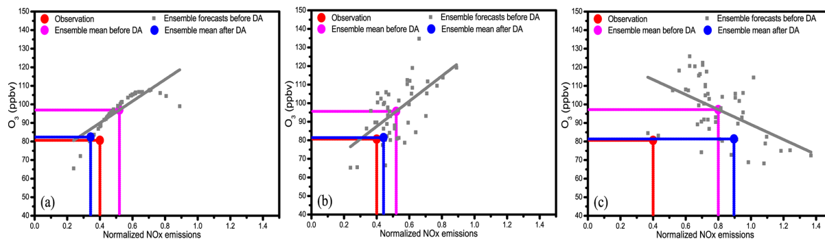
Figure 6. (a–c) O 3 concentrations (ppbv) and NO x emissions (no unit, normalized by the true NO x emission) before and after data assimilation and their ensemble samples before DA at 12:00 LT on 12 August 2008 in the three ideal DA experiments. The NO 2 photolysis rate is assumed to be overestimated by 20 %. (a) The prior NO x emission is overestimated by 30 % and adjusted by the DA, but the uncertainty of the NO 2 photolysis rate is not included (there are no perturbations of the NO 2 photolysis rate) in the DA. (b) The same as the DA experiment in (a), but the uncertainty of the NO 2 photolysis rate is taken into account by perturbing it. (c) The same as the DA experiment in (b), but the bias in the prior NO x emission is increased to 100 %. The magenta dot, the gray squares, the gray line, the red dot, and the blue dot represent the same information as in Fig. 4.
