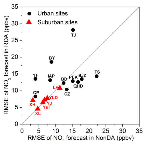
Figure 2. Comparison of the RMSE (ppbv) of 1h NO 2 forecasts at the 17 stations of Beijing and its surrounding areas during the period of 00:00 local time (LT) 9 August to 00:00 LT, 23 August in 2008 in the RDA experiments and those in the reference (NonDA) experiment with a free run of the model. The comparisons at urban sites are denoted by the dots and those over suburban stations are represented by the triangles. The abbreviations of the station names are displayed close to the marks. The number of the valid observations used for the calculation is 336 at QHD, SJZ, TS, IAP, LF, YF, and XH, and the numbers are 292, 226, 326, 317, 326, 320, 333, 321, 311, and 323 at BD, PEK, BY, CZ, CP, TJ, XL, YJ, YLD, and YuF, respectively.
