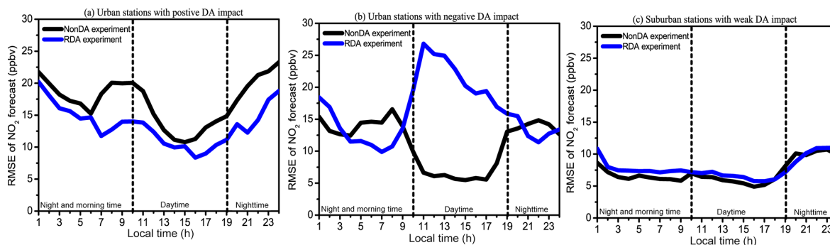
Figure 3. Daily variation of the 1 h NO 2 forecast RMSE (ppbv) in the RDA experiments (blue line) and the reference (NonDA) experiment with a free run of the model (black line) over (a) urban stations (CZ, PEK, QHD, SJZ, and TS) with positive DA impacts; (b) urban sites (BY, CP, IAP, TJ, and YF) with negative DA impacts; (c) suburban stations (LF, XH, YLD, YJ, and YuF) with weak DA impacts.
