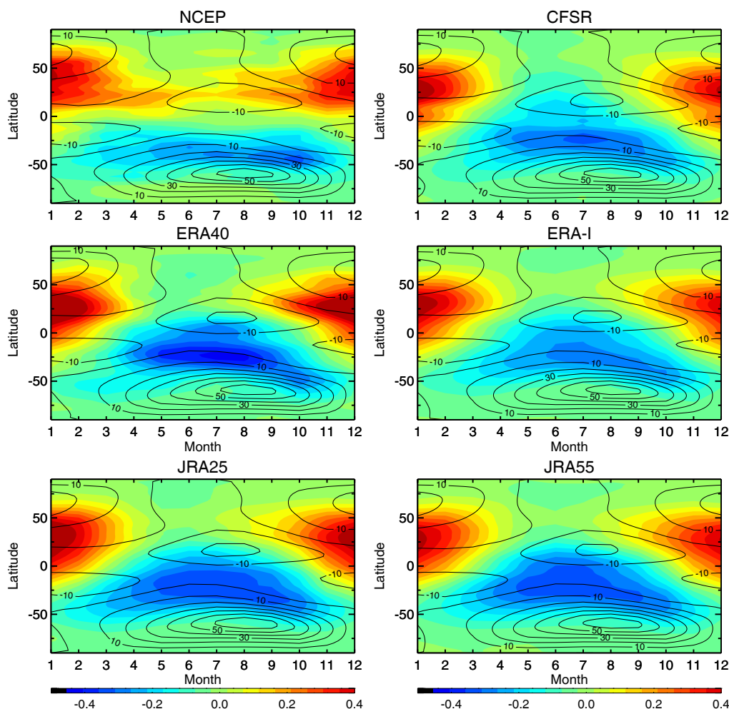
Figure 4. Seasonal variation of the mass stream function (color contours, in 10^{10} \text{ kg s}^{-1} ) and zonal mean zonal wind (black contour lines, with intervals of 10 \text{ m s}^{-1} ) at 560 K.
