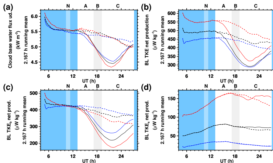
Figure 9. Wind speed and the diurnal cycle. Time series from simulations M^- (blue), M^0 (black), M^+ (red), solid curves, and from simulations M^-_{\text{dark}} (blue), M^0_{\text{dark}} (black), M^+_{\text{dark}} (red), dashed curves. The cloud base water flux in updrafts is given per horizontal surface area of the domain. A low-pass (running mean) filter was applied where indicated to reduce noise.
