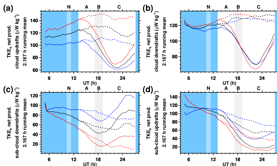
Figure 10. Wind speed and the diurnal cycle. Time series from simulations M^- (blue), M^0 (black), M^+ (red), solid curves, and from simulations M^-_{\text{dark}} (blue), M^0_{\text{dark}} (black), M^+_{\text{dark}} (red), dashed curves. TKE production rates are given per total boundary layer air mass. A low-pass (running mean) filter was applied where indicated to reduce noise.
