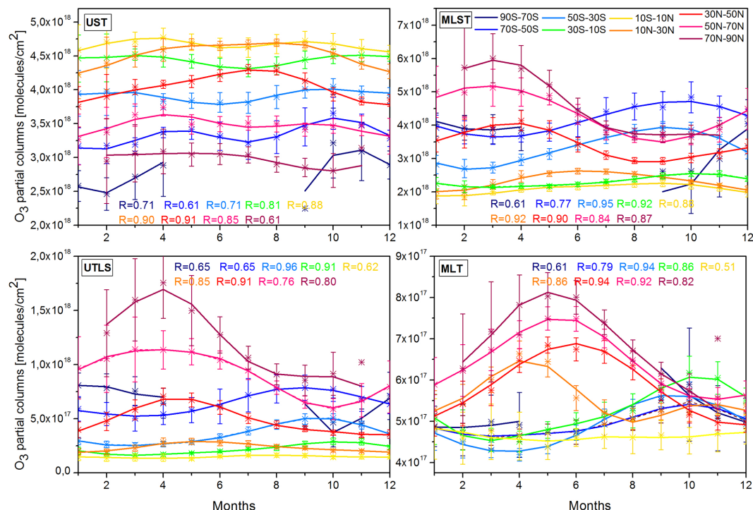
Figure 7. Monthly medians of measured (scatters) and of fitted (line) IASI \text{O}_3 columns averaged over the period 2008–2013, for the UST, MLST, UTLS and MLT layers and for each 20^\circ latitude band (colour scale in the top-right panel). The fit is based on daily medians. Error bars give the 1\sigma standard deviation relative to the monthly median values. Correlation coefficients ( R ) between the daily median observations and the fit are also indicated. Note that the scales are different.
