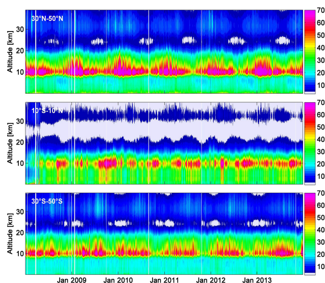
Figure 5. Daily IASI O 3 variability (%), expressed as [\sigma(\text{O}_3(t))/\text{O}_3(t)] \times 100\% , where \sigma is the standard deviation, as a function of time and altitude in three latitude bands: 30–50° N (top), 10° S–10° N (middle) and 30–50° S (bottom).
