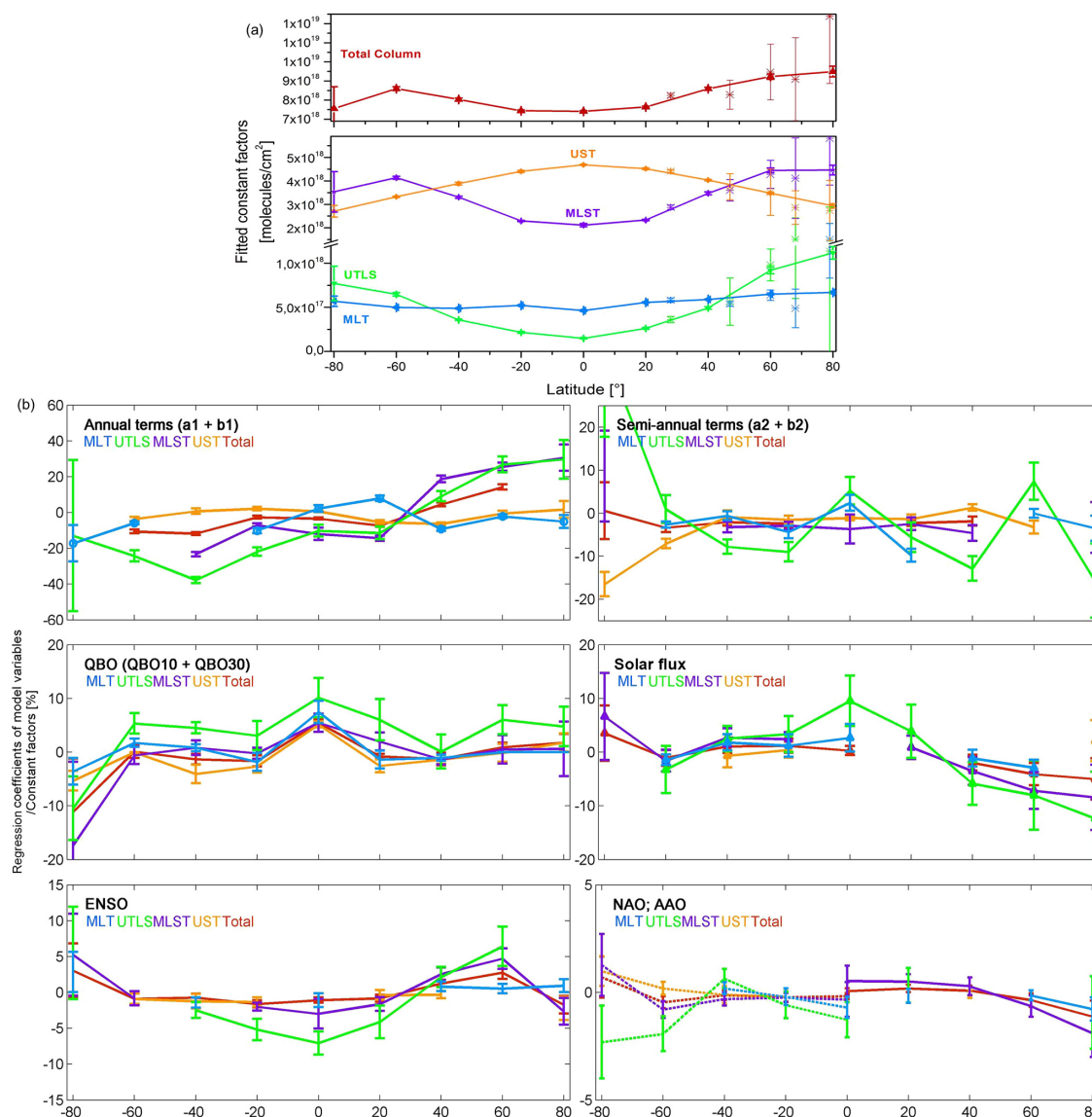
Figure 8. (a) Fitted constant factors (Cst; see Eq. 1, Sect. 3) from the 6-year IASI daily O 3 time series for the 20° latitude belts, separately given for the four layers and for the total column. The stars correspond to the constant factors fitted above ground-based measurement stations: Ny-Ålesund (79° N), Kiruna (68° N), Harestua (60° N), Jungfraujoch (47° N) and Izana (28° N). (b) Regression coefficients of the variables retained by the stepwise procedure, given in % as [\text{regression\_coefficient}/\text{fitted\_cst}] \times 100\% . Identification for the variables: annual (top left) and semi-annual variation (top right) terms, QBO at 10 and 30 hPa (bottom left) and solar flux (bottom right). Note that the scales are different. The associated fitting uncertainties (95 % confidence limits) are also represented (error bars).
