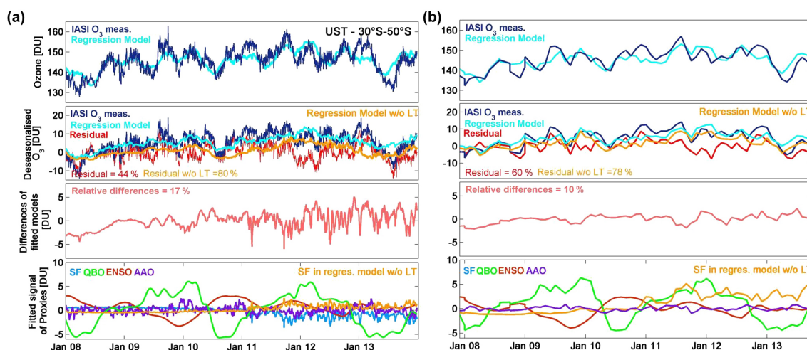
Figure 9. Daily (a) and monthly (b) time series of \text{O}_3 measurements and of the fitted regression model in the UST for the 30\text{--}50^\circ\text{S} latitude band (top row), of the deseasonalised \text{O}_3 (second row), of the difference of the fitted models with and without the linear term (third row) and of the fitted signal of proxies [regression_coefficient \times proxy]: SF (blue), QBO ( \text{QBO}^{10} + \text{QBO}^{30} ; green), ENSO (red) and AAO (purple) (bottom) (given in DU). The averaged residuals relative to the deseasonalised IASI time series are also indicated (%).
