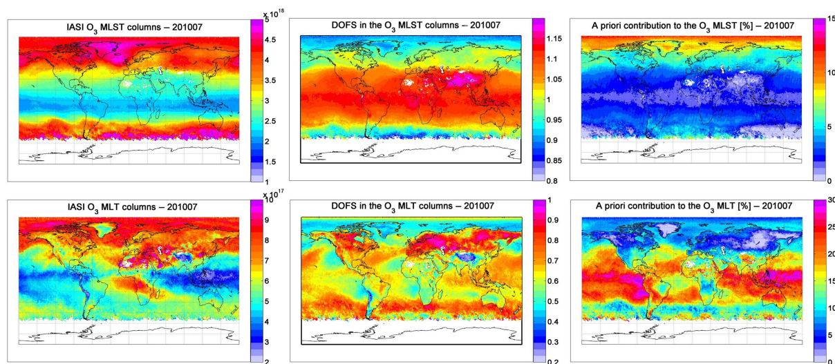
Figure 2. Distributions of (a) \text{O}_3 columns, (b) DOFS and (c) a priori contribution (given as a %) in the ground–300 hPa (MLT) and 150–25 hPa (MLST) layers for IASI \text{O}_3 , averaged over July 2010 daytime data. Note that the scales are different.
