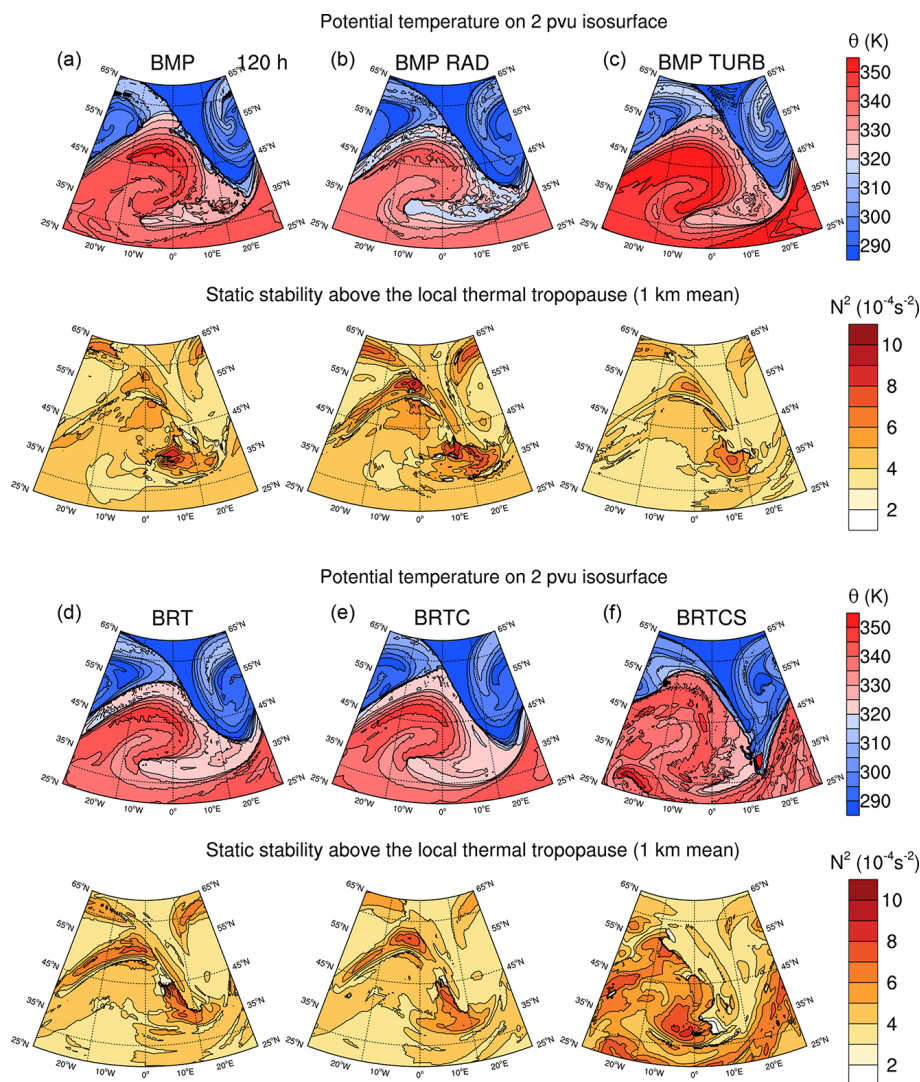
Figure 8. Dynamical and thermodynamical state of baroclinic life cycles after 120 h of model integration. In the upper rows of the six panels, the distribution of potential temperature \Theta (in K) on the dynamical tropopause is depicted, while the lower rows show the distribution of static stability N^2 (in 10^{-4} \text{ s}^{-2} ) averaged over the first kilometer above the thermal tropopause for (a) BMP, (b) BMP RAD, (c) BMP TURB, (d) BRT, (e) BRTC, and (f) BRTCS.
