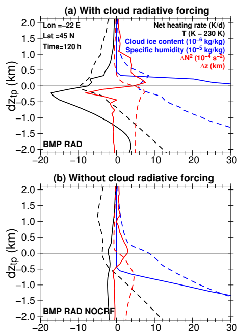
Figure 13. Tropopause-based vertical profiles through an ice cloud along the central latitude at 120 h for (a) a simulation with cloud radiative forcing (BMP RAD) and (b) a simulation without cloud radiative forcing (BMP RAD NOCRF). Solid lines show net radiative heating (in \text{K d}^{-1} , scaled for better comparability, black), cloud-ice content (in 10^{-6} \text{ kg kg}^{-1} , blue), and \Delta N^2 (in 10^{-4} \text{ s}^{-2} , red). Dashed lines show temperature (in \text{K} - 230 \text{ K} , black), specific humidity (in 10^{-5} \text{ kg kg}^{-1} , blue), and \Delta z (in km, red). dz_{tp} is the distance to the height of the thermal tropopause.
