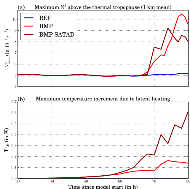
Figure 5. Temporal evolution between 30 and 80 h after simulation start of (a) the maximum static stability N^2_{\max} (in 10^{-4} \text{ s}^{-2} ) above the thermal tropopause and (b) the maximum temperature increment due to latent heating T_{LH} (in K) in the model domain for REF (blue lines), BMP (red lines), and BMP SATAD (dark red lines).
