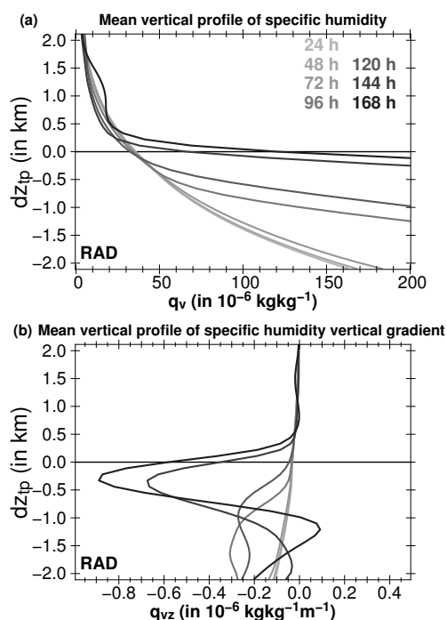
Figure 4. Instantaneous thermal tropopause-based domain mean values of (a) specific humidity q_v (in 10^{-6} \text{ kg kg}^{-1} ) and (b) the vertical gradient of specific humidity \partial q_v / \partial z (in 10^{-6} \text{ kg kg}^{-1} \text{ m}^{-1} ) for RAD. The domain mean is calculated within 25\text{--}65^\circ latitude and the entire zonal domain. dz_{tp} is the distance to the height of the thermal tropopause. The intensity of the gray colors indicates the time since model start in 24 h intervals.
