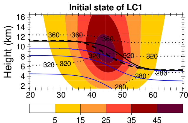
Figure 1. Meridional cross section of the initial state at the center of the model domain: the zonal wind U is color-coded for values of 5, 15, 25, 35, and 45 \text{ m s}^{-1} ; the potential temperature \Theta is shown by the black dotted lines for 280, 320, and 360 K (from bottom to top); the water vapor mixing ratio is shown by the blue lines for values of 2.0, 0.2, and 0.02 \text{ g kg}^{-1} (from bottom to top); the location of thermal tropopause is indicated by the solid thick black line and also separates the region of tropospheric values ( N^2 < 1.5 \times 10^{-4} \text{ s}^{-2} ) from stratospheric values ( N^2 \sim 4.0 \times 10^{-4} \text{ s}^{-2} ) of static stability; the location of the dynamical tropopause, defined as the isosurface of potential vorticity Q = 2.0 \text{ pvu} , is shown by the dashed thick line.
