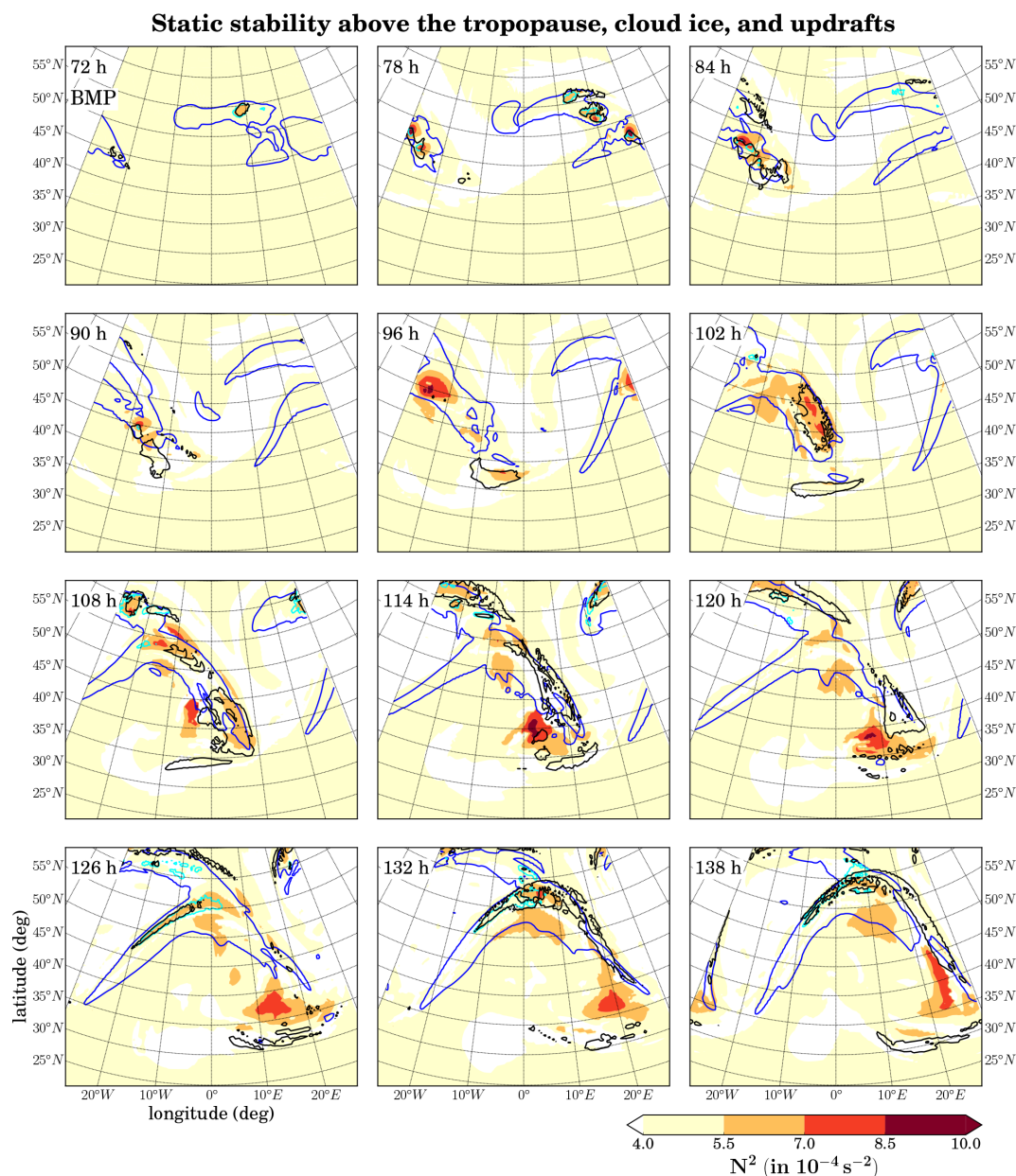
Figure 9. Static stability N^2 (color-coded, in 10^{-4} \text{ s}^{-2} ) above the thermal tropopause, \Delta z (black lines, in 2.5 km), column integrated cloud-ice content tq_i (blue lines, in 0.01 \text{ kg m}^{-2} ), and tropopause close column integrated cloud-ice content tq_{i,tp} (cyan lines, in 0.001 \text{ kg m}^{-2} ). Tropopause close means the region between the thermal tropopause and 500 m below. The distribution is shown for BMP between 72 and 138 h after simulation start in a 6-hourly interval.
