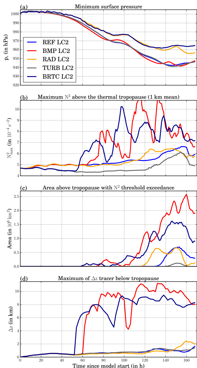
Figure 15. Temporal evolution over the entire simulated life cycles of (a) the minimum surface pressure p_s (in hPa), (b) the maximum static stability N^2_{\max} (in 10^{-4} \text{ s}^{-2} ) above the thermal tropopause, (c) the area A_{5.5} (in 10^6 \text{ km}^2 ) of N^2 threshold exceedance above the thermal tropopause (with a threshold of N^2 = 5.5 \times 10^{-4} \text{ s}^{-2} ), and (d) the maximum of the \Delta z tracer (in km) in a 500 m thick layer below the thermal tropopause. The colored lines indicate the following simulations: REF LC2 (blue), BMP LC2 (red), RAD LC2 (orange), TURB LC2 (gray), and BRTC LC2 (dark blue).
