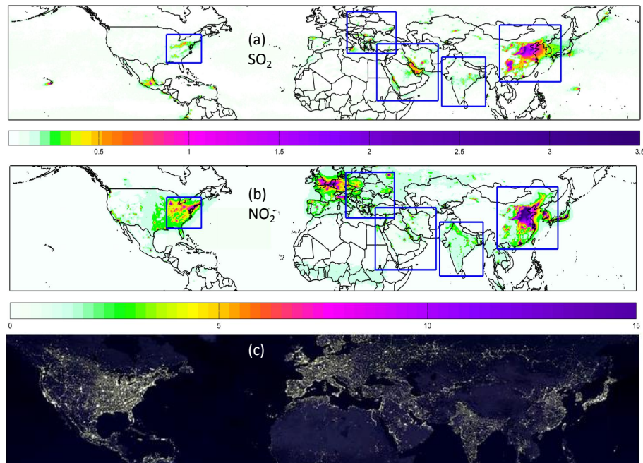
Figure 1. OMI-derived maps of PBL SO 2 in Dobson Units [DU] (a) and tropospheric NO 2 columns in [10 15 molecules cm -2 ] (b) for 2005–2007 show enhanced pollution levels around major cities and industrial centers, seen also in the “Earth at Night” (city lights) map (c) , courtesy of Aura EPO team.
