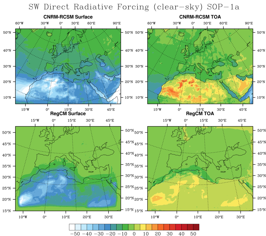
Figure 29. Averaged surface and TOA SW DRF simulated in clear-sky conditions and over the SOP-1a period by the CNRM-RCSM and RegCM models.
