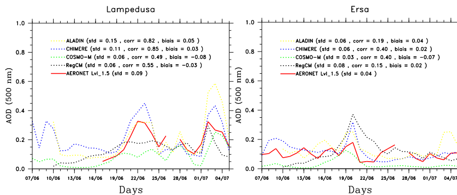
Figure 28. Times-series of AOD comparisons between AERONET/PHOTONS observations and COSMO-MUSCAT, CHIMERE, CNRM-RCSM and RegCM model outputs over the two stations of Ersa and Lampedusa.
