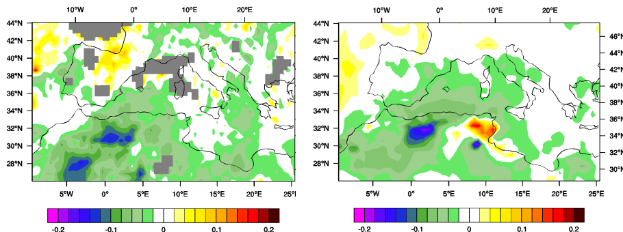
MISR observations
