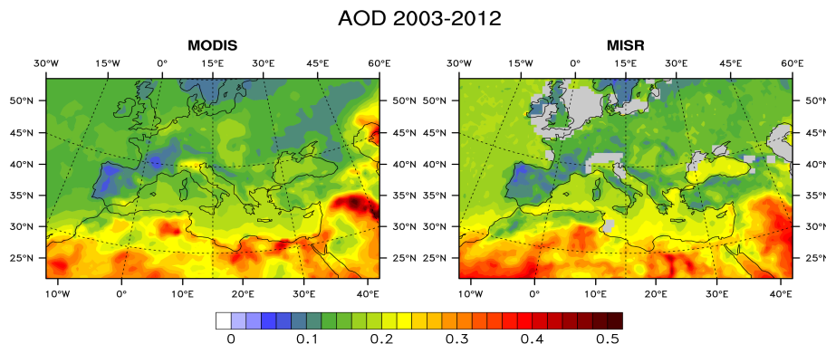
Figure 1. Aerosol Optical Depth (at 550 nm) derived from MODIS and MISR satellites for the 2003 to 2012 period.
