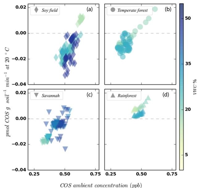
Figure 9. The mixing ratio of COS exiting the incubation chamber versus COS fluxes after water addition at 20 °C.
