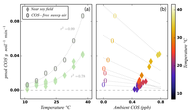
Figure 4. Net COS exchange over temperature from a soil sample taken near the original soy field site: fluxes observed under ambient sweep air and COS-free sweep air conditions with exponential least-squares regression lines (a), and the relationship between ambient chamber COS concentrations and observed fluxes with linear least-squares regression lines (b).
