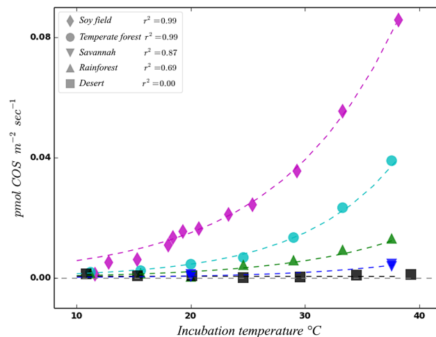
Figure 11. Observations of COS fluxes from air-dried soils over a range of temperatures. Air-dried soils experience negligible COS uptake; the net fluxes here are assumed to be soil COS production only. Equation (4) was used to curve-fit the relationship between temperature and soil COS production with least-squares regression. The r^2 values of this attempt are shown in the figure legend.
