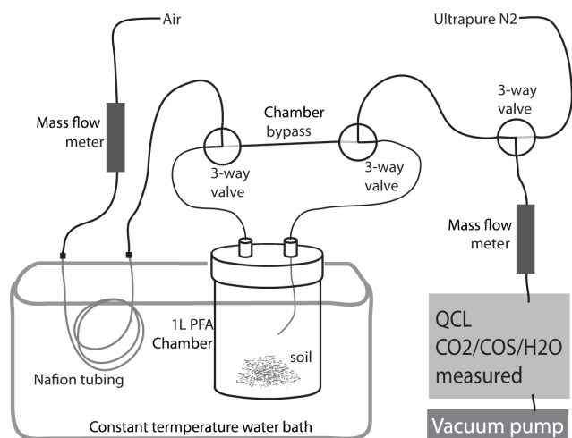
Figure 3. The experimental setup for laboratory-based soil incubation experiments. The Nafion tubing was placed in a container of water and used to humidify the incoming gas stream. Three-way valves were used to switch between analyzing a nitrogen stream, the gas stream that flowed through the chamber ( C_f , orientation of valves illustrated above), and the gas stream bypassing the chamber ( C_i ).
