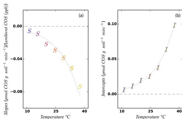
Figure 5. Slopes (a) and intercepts (b) of the linear least-squares regression lines in Fig. 4b and their exponential linear least-squares regression relationship with incubation temperature (dotted lines).
