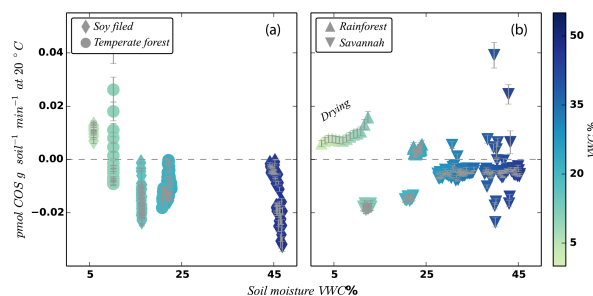
Figure 8. COS flux observations at 20 °C after soil water content manipulation for soy field and temperate forest soils (a) and rainforest and savannah soils (b). A rainforest soil sample in (b) was intentionally dried out by removing the Nafion tubing in the experimental setup (see Fig. 3).
