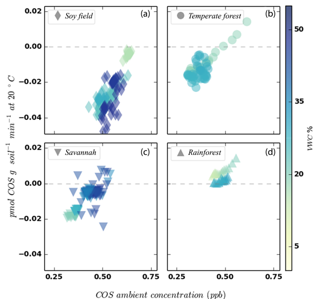
Figure 10. Soil COS mole fractions and soil COS flux after water addition at 20 °C with subtraction of anticipated COS production shown in Fig. 11.
