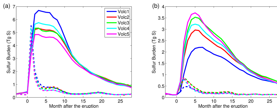
Figure A2. \text{SO}_2 (dashed lines) and sulfate (solid lines) burden after the eruption on (a) Northern Hemisphere and (b) Southern Hemisphere. Note different the scales on the y axes.
