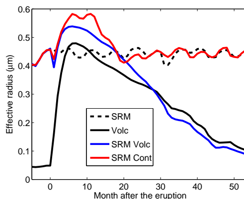
Figure 3. Mean effective radius in the different scenarios between 20^{\circ} N and 20^{\circ} S latitudes and between 20 and 25 km altitude levels.
