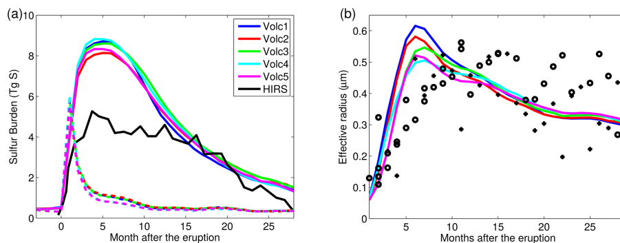
Figure A1. (a) Global \text{SO}_2 (dashed lines) and particulate sulfate (solid lines) burdens after a simulated volcanic eruption in July compared to sulfate observations from HIRS satellite after the 1991 Pinatubo eruption (black). (b) Zonal mean effective radius at 53° N latitude after the simulated July eruption compared to lidar measurements at Laramie 41° N (dots) and Geesthacht 53° N (crosses) after the Pinatubo eruption (Ansmann et al., 1997). In both panels the results are shown for altitude range 16–20 km. The different coloured lines show results from the five members of the simulated ensemble (simulations Volc1, ..., Volc5).
