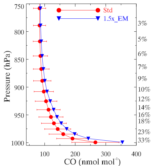
Figure 10. Monthly average vertical profile of CO over Chennai during June from Std and 1.5x_EM simulations. The resulting enhancement in CO is also indicated in percentages along the right axis.
