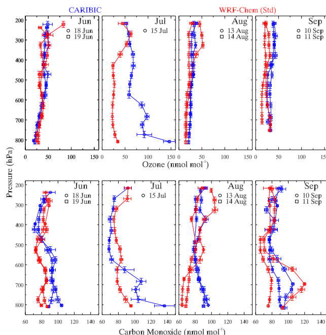
Figure 2. Comparison of ozone and carbon monoxide profiles from WRF-Chem simulations (Std, red lines) with the CARIBIC observations (blue lines) during June, July, August and September 2008. Model output has been spatially and temporally interpolated along the CARIBIC flight tracks. Only data collected during the aircraft descent are shown here (see Sect. 4.1.1 for details).
