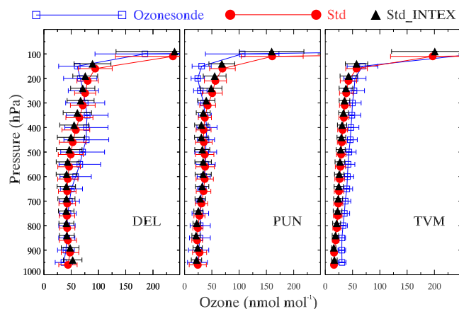
Figure 5. Comparison of average ozone mixing ratios during the summer monsoon (June–September) from Std and Std_INTEX WRF-Chem simulations with the ozonesonde observational climatology during 2006–2009 period over Delhi (DEL), Pune (PUN) and Thiruvananthapuram (TVM).
