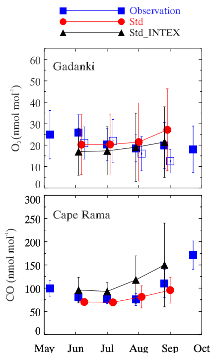
Figure 8. Comparison of WRF-Chem simulated surface ozone and CO with the ground-based measurements at Gadanki (79.2° E, 13.5° N; Naja and Lal, 2002) and Cape Rama (73.8° E, 15.1° N). Open blue symbols for Gadanki show observations from another study (Renuka et al., 2014). Comparison with Std_INTEX simulation is indicated in black.
