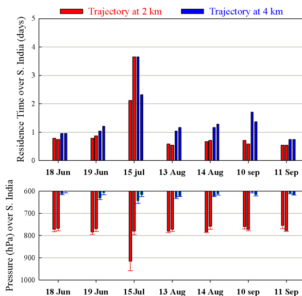
Figure 12. Residence time of air masses over the southern Indian region on all CARIBIC measurement days calculated from the back-trajectories at 2 and 4 km above Chennai. The mean pressure along the trajectory over southern India is also shown.
