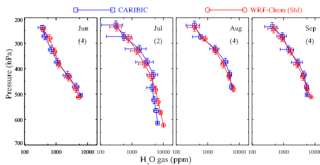
Figure 4. Comparison of monthly average H_2O gas (ppm) from standard WRF-Chem simulations (Std) with the CARIBIC observations during June, July, August and September 2008. Numbers in brackets denote the number of observational profiles in the respective month. Model output has been spatially and temporally interpolated along the CARIBIC flight tracks. Note the logarithmic scale on the x axis.
