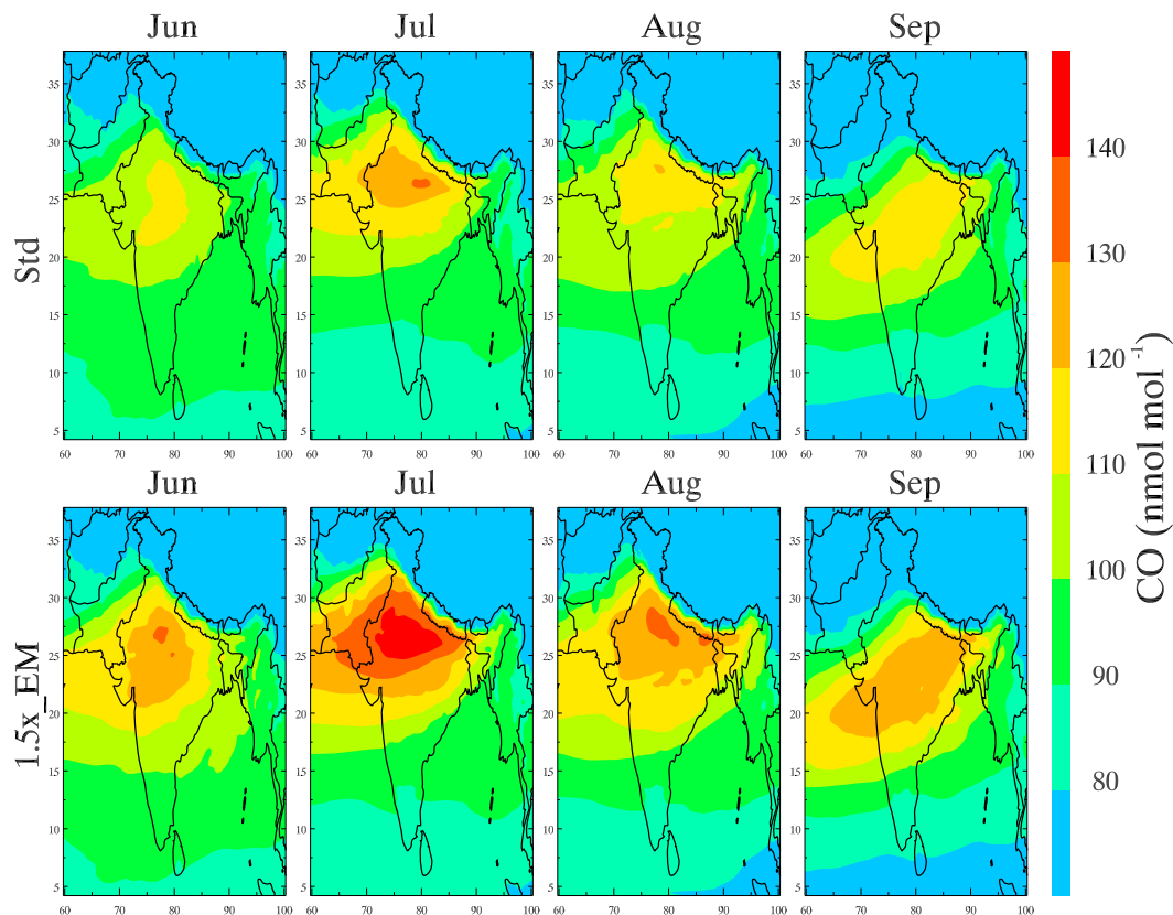
Figure 9. Comparison of monthly average horizontal distribution of CO in the upper troposphere (116 to 211 hPa) over India from the Std simulation (top panel) and 1.5x_EM simulation (bottom panel) during June, July, August and September 2008.
