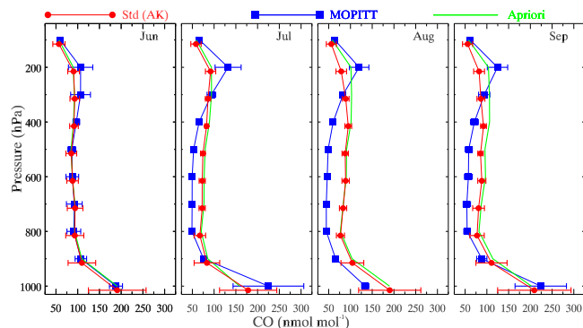
Figure 6. Comparison of monthly average CO from WRF-Chem simulations (Std) with the MOPITT retrievals over Chennai during the 4 months of the summer monsoon period of the year 2008. The MOPITT averaging kernel and the a priori profile have been applied to the WRF-Chem output, denoted by Std (AK). MOPITT a priori profile is also shown for comparison.
