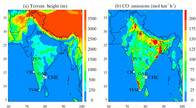
Figure 1. (a) The simulation domain of WRF-Chem covering the South Asian region at a spatial resolution of 30 \times 30 km, including topography map. (b) Anthropogenic emissions of CO over the South Asian region for June 2008 from the HTAP v2.2 emission inventory. The location of Chennai (CHE) is shown over which the profiles have been measured as a part of the CARIBIC program. Cape Rama (CR) and Gadanki (GAD) are two additional sites for which ground-based measurements have been used. The three ozonesonde stations Delhi (DEL), Pune (PUN) and Thiruvananthapuram (TVM) are also shown.
