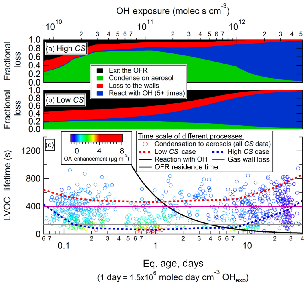
Figure 5. Fractional fates of loss of LVOCs to OFR walls, condensation to aerosols, reaction with OH to produce volatile products, or exiting the OFR to be lost on sampling line walls as a function of photochemical age for (a) high-CS and (b) low-CS cases; (c) LVOC lifetimes for each of these pathways. Lifetime for condensation to aerosols is shown for all data points (colored by OA enhancement after oxidation) using CS calculated from SMPS measurements.
