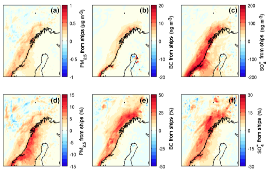
Figure 10. 15-day average (00:00 UTC 11 July 2012 to 00:00 UTC 26 July 2012) of (top) absolute and (bottom) relative surface enhancements (CTRL – NOSHIPS) in (a, d) PM_{2.5} , (b, e) BC and (c, f) SO_4^{2-} due to ship emissions in northern Norway from STEAM2.
