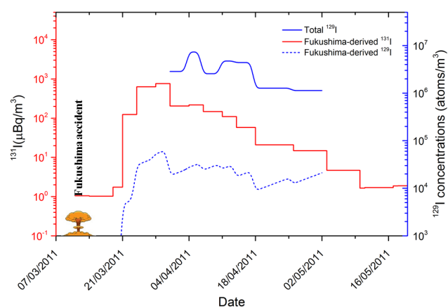
Figure 7. ^{131}\text{I} radioactivity (red, Nielsen et al., 2011), ^{129}\text{I} concentrations (blue) in aerosols from Risø, Denmark after the Fukushima accident. The Fukushima-derived ^{129}\text{I} concentrations are calculated based on ^{129}\text{I}/^{131}\text{I} atomic ratio of 16.0 \pm 2.2 deduced from Fukushima-affected aerosol samples (Xu et al., 2015).
