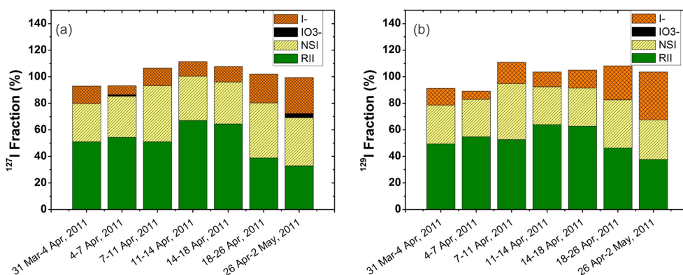
Figure 5. Distribution of iodine species in the aerosol samples for ^{127}\text{I} (a) and ^{129}\text{I} (b), compared with the measured concentrations of total ^{127}\text{I} and ^{129}\text{I} in bulk aerosols.
