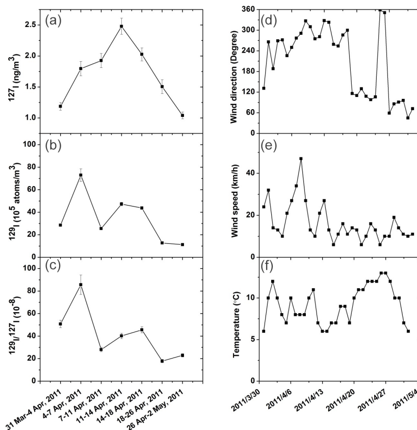
Figure 3. Variation of ^{127}\text{I} concentrations (a), ^{129}\text{I} concentrations (b), ^{129}\text{I} / ^{127}\text{I} ratios in aerosols (c), wind direction (d), wind speed (e), and temperature (f) during the sampling period. The historical meteorological data, including temperature, wind direction, and wind speed were obtained from the observation station of Hangarvej in Roskilde, Denmark ( 55.594^\circ \text{N} 12.128^\circ \text{E} ) based on 41 m a.s.l. (above sea level) (Weather Wunderground webpage, 2015).
