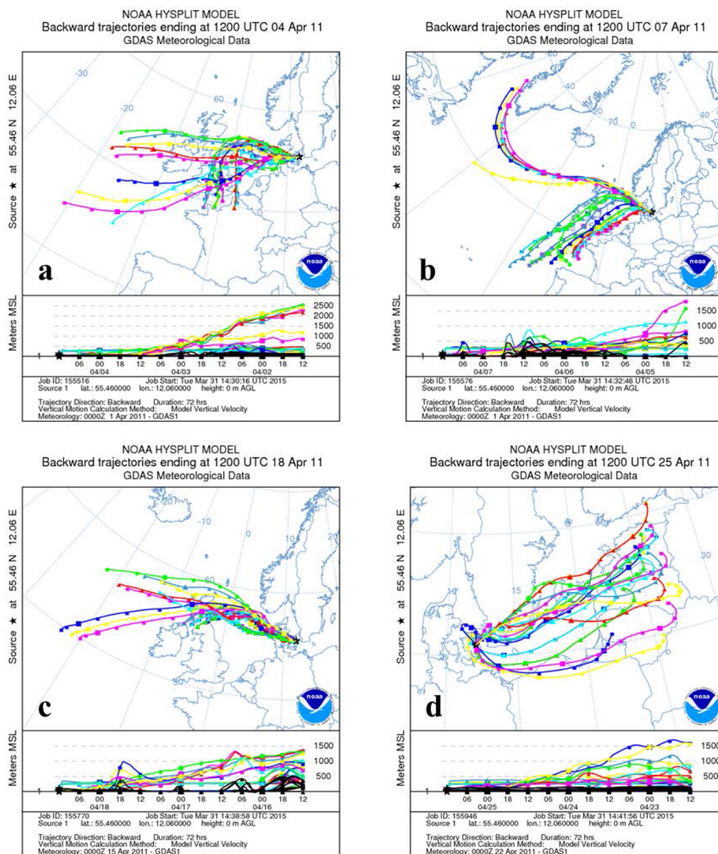
Figure 6. The 72 h (3 days) air mass back trajectories for starting altitudes of 0 m above ground level (a.g.l.) calculated from the FNL database of the National Ocean and Atmospheric Administration (NOAA) and simulated by using the Hybrid Single-Particle Lagrangian Integrated Trajectory (HY-SPLIT) model. 31 March–4 April (a), 4–7 April 2011 (b), 14–18 April (c) and 21–25 April 2011 (d).
