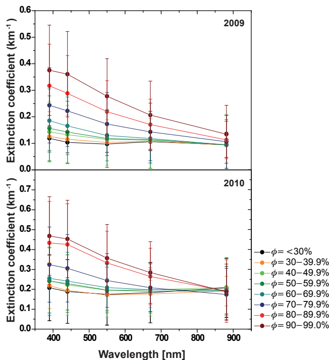
Figure 12. The mean extinction coefficient spectrum for eight relative humidity classes (indicated by different colors) for the years 2009 (top) and 2010 (bottom). Vertical bars indicate the SD for each of the shown five extinction coefficients (for five wavelengths) for a given humidity interval.
