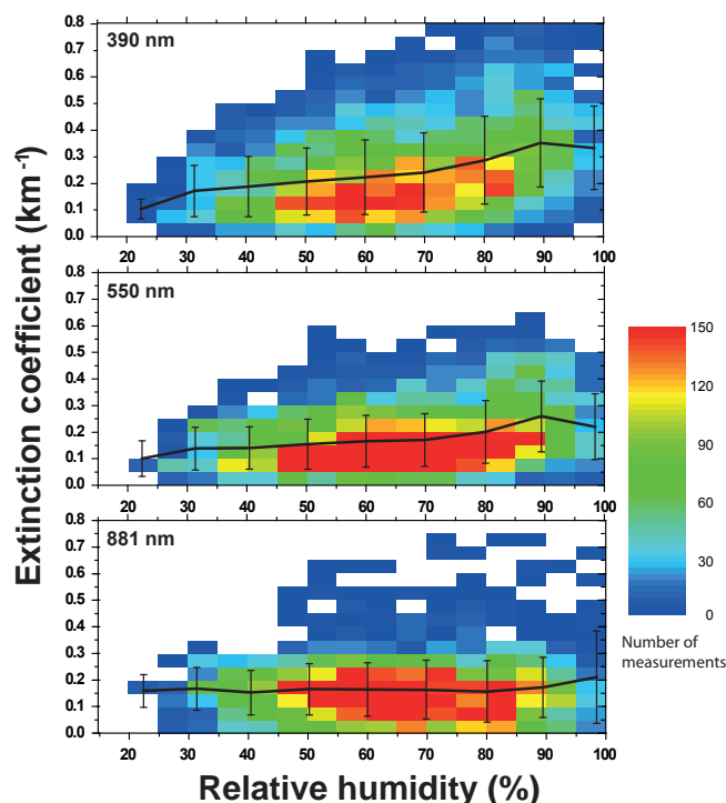
Figure 2. Measured particle extinction coefficients for the wavelengths of 390 nm (top), 550 nm (center) and 881 nm (bottom) as a function of relative humidity. The color scale indicates how frequently a given extinction coefficient was measured during the 2009–2012 period. Mean values (bold lines) of extinction coefficients and corresponding standard deviation (SD, vertical bars) are shown for 10 % humidity intervals.
