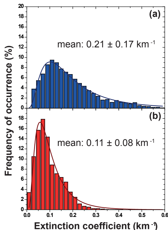
Figure 4. (a) Frequency distribution of ambient 550 nm particle extinction coefficient observed with SÆMS at Leipzig from 2009 to 2012; (b) same distribution after correction of the particle water uptake effect, i.e., after normalization of all values to 0 % relative humidity by means of Eq. (3) with the parameter for urban aerosol derived from the 4-year SÆMS study. The 2009–2012 mean value and respective SD are given as numbers.
