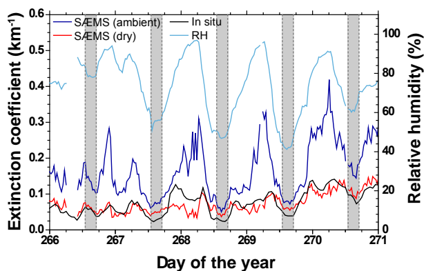
Figure 9. Comparison of 550 nm extinction coefficients measured with SÆMS (ambient, dark blue) and computed from dry particle size distributions (black) measured in situ at the roof of the TROPOS building from 24 to 29 September 2009. The humidity-corrected SÆMS (dry, 0 % relative humidity) extinction time series is shown as a red curve. Relative humidity is given in addition as a light blue line. Gray shaded areas indicate the 13:00–17:00 UTC periods during which the PBL is assumed to be well mixed; PBL depth takes its maximum, and relative humidity and particle extinction take their minimum during sunny days (days 267, 268, 269).
