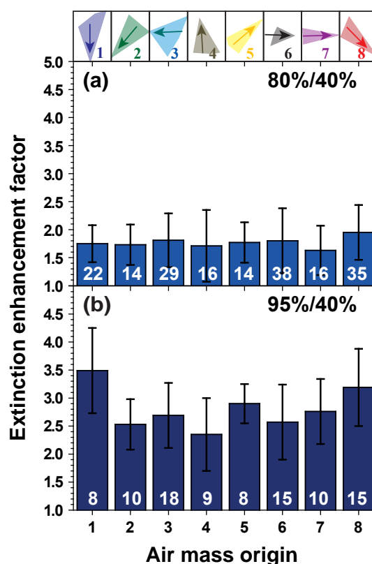
Figure 8. Particle extinction enhancement factors for 550 nm (80–40 and 95–40 % RH enhancement) observed from days with occurring humidity variations between at least 40 and 80 % RH (a) and only from days with variations between at least 40 and 95 % RH (b) separated for the eight air-mass transport regimes. The 4-year mean values and SD are given.
