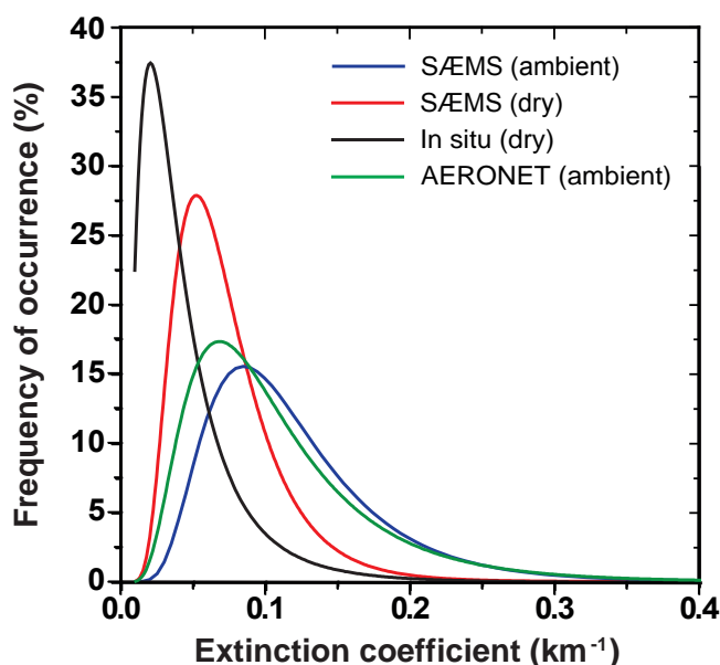
Figure 10. Frequency of occurrence of 550nm particle extinction coefficient measured with SÆMS (ambient) at TROPOS, Leipzig, between 13:00 and 17:00 UTC of each day in the year of 2009 (blue line). For comparison, the respective distribution for the PBL-mean extinction coefficient (ambient, green) is shown. These values are derived from AERONET sun photometer observations of the 500nm particle optical depth divided by the PBL depth, which was estimated from GDAS1 model data. The red SÆMS (dry) curve shows the distribution of humidity-corrected SÆMS 550nm particle extinction values (for 0 % relative humidity). The black distribution (in situ, dry) shows the 550nm extinction values calculated from in situ observations of the dry particle size distribution at the roof of the TROPOS building exclusively for the time period from 13:00 to 17:00 UTC.
