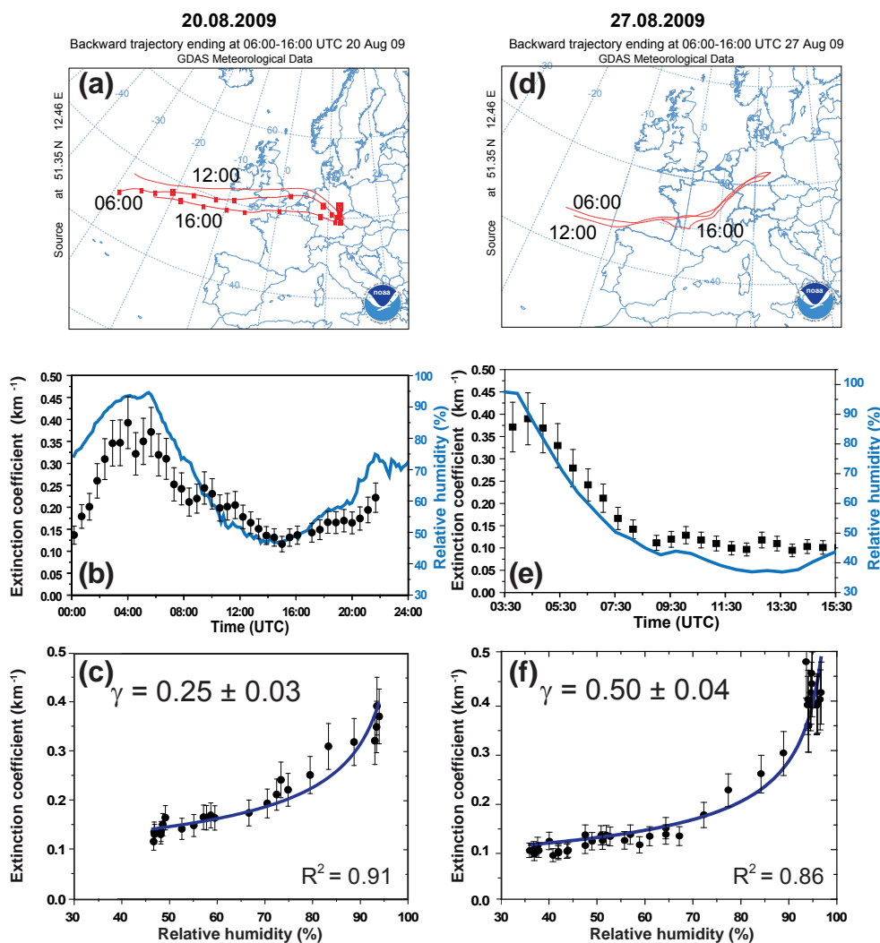
Figure 5. SÅEMS observations on (left) 20 August 2009 and (right) 27 August 2009. Almost constant horizontal transport of polluted air from westerly to southwesterly directions is indicated by 4-day HYSPLIT backward trajectories (a, d, arrival height of 500m). The temporal variation of the 550 nm particle extinction coefficient with relative humidity is shown in (b) for 20 August 2009 and in (e) for 27 August 2009, and the corresponding relationship between ambient extinction coefficient and relative humidity is presented in (c, f). The curves fitted to the data points in (c, f) are obtained with Eq. (3). The coefficient of determination R^2 for each fit is given as number.
