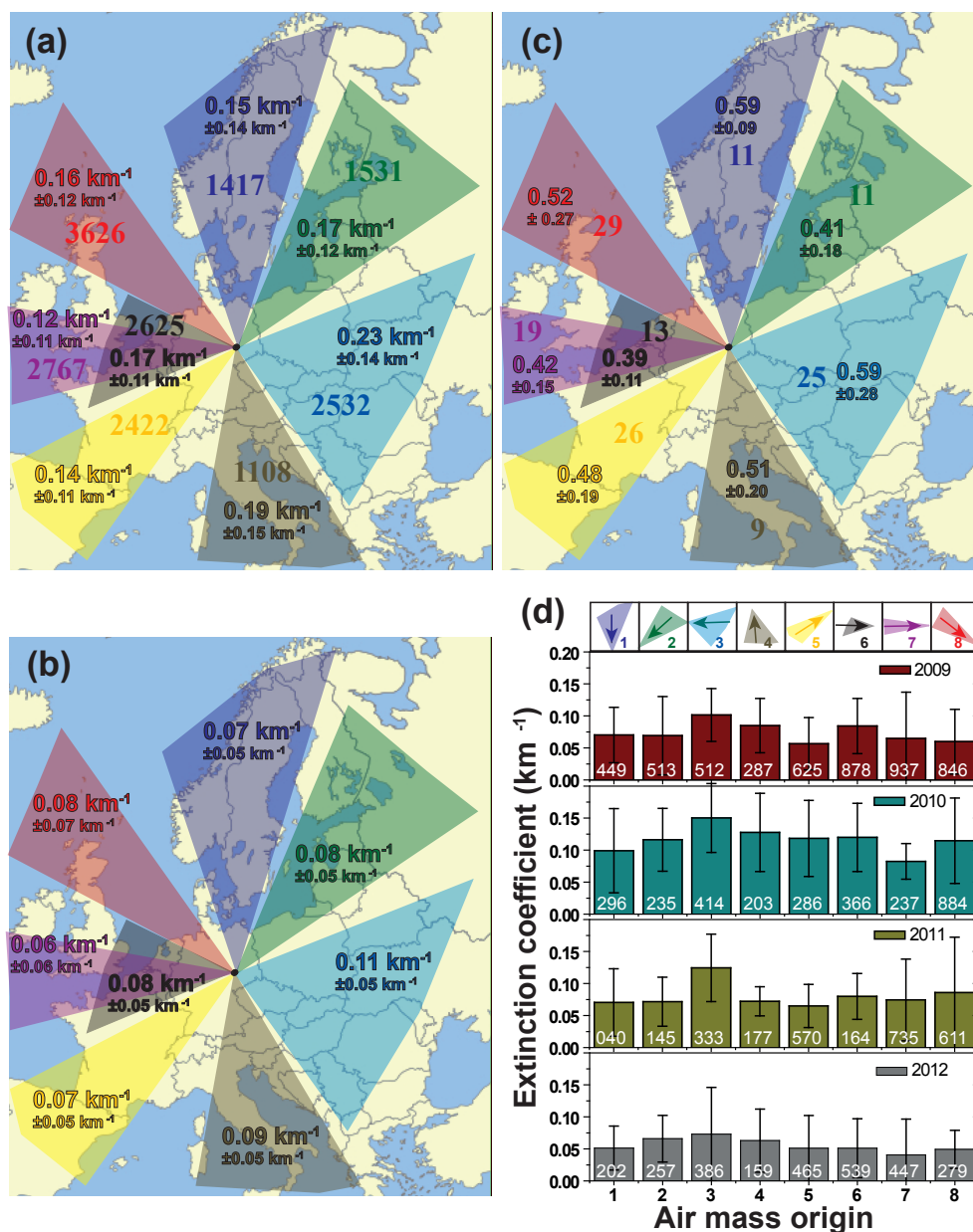
Figure 7. (a) Extinction coefficient for 550 nm (mean value, SD, number of measurements) for eight defined air-mass transport regimes based on SÆMS observations from 2009 to 2012, (b) same as (a), except prior to averaging all individual cases were normalized for dry conditions (RH = 0 %) by use of the derived cluster mean parameter \gamma (c) and (c) hygroscopic exponent \gamma for 550 nm (mean value and SD, computed with Eq. 3) for the eight air-mass transport regimes derived from SÆMS observations from 2009 to 2012. Numbers of available cases per cluster are given in addition, and (d) same as (b), but separately for dry conditions (RH = 0 %) for each year of the period from 2009 to 2012.
