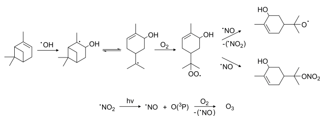
Figure 1. The formation of atmospheric organic nitrates and ozone from the gas phase oxidation of \alpha -pinene, initiated by the OH radical.
