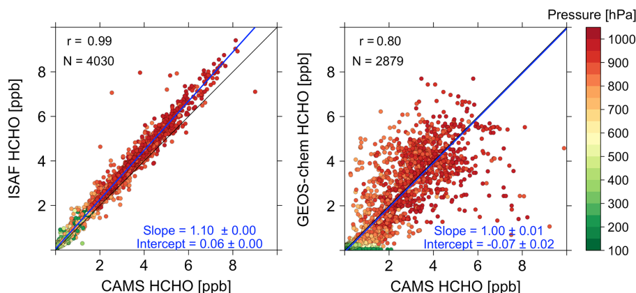
Figure 2. Comparisons between HCHO measurements from the CAMS and ISAF instruments aboard the SEAC 4 RS aircraft, and simulated by GEOS-Chem, for the southeast US flight tracks (box in Fig. 1). The left panel compares 1 min measurements from CAMS and ISAF. The right panel compares GEOS-Chem and CAMS HCHO. Here and elsewhere for model–observation comparisons, HCHO observations along the flight tracks are averaged onto the GEOS-Chem grids ( 0.25^\circ \times 0.3125^\circ , 47 vertical layers) and time steps (10 min). HCHO data points are colored by atmospheric pressure. Slopes and intercepts of reduced major axis (RMA) regressions are shown along with the correlation coefficient ( r ), sample size ( N ), RMA regression line (in blue) and 1 : 1 line.
