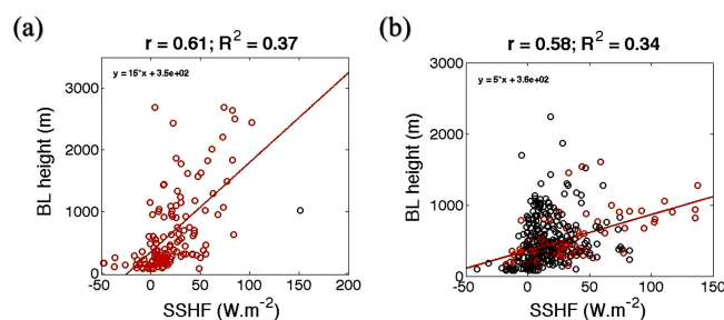
Figure 7. The scatter plot of SSHF and BL height during (a) the uplift regime, and (b) the stratus regime. The linear relationship between the SSHF and BL height derived using the least squares method of curve-fitting for (a) all cases (except one outlier indicated by black marker), and (b) cases with surface wind speeds exceeding 9.8 \text{ ms}^{-1} (indicated by red markers). The correlation coefficient and the coefficient of multiple determination for each linear relationship is denoted by r and R^2 , respectively. Note that the outlier in the uplift regime is an observation point with maximum \Delta T , which has no influence on r . Conversely, the red markers in the stratus regime are observations with maximum surface wind speeds, which have a positive influence on r . See Sect. 4.2 for explanation.
