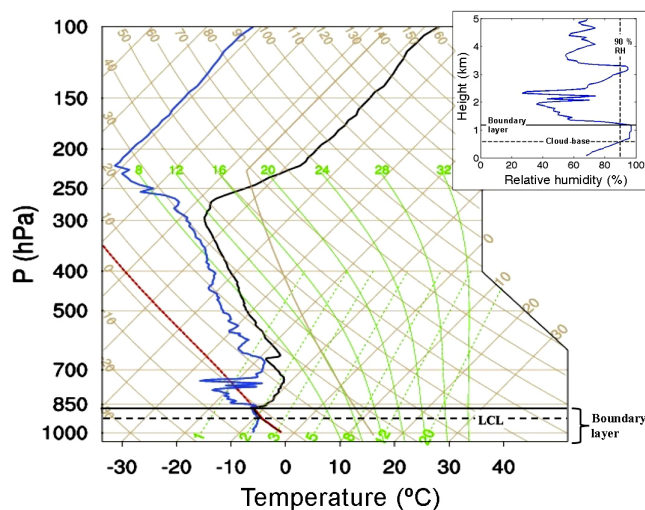
Figure 2. Skew T -log P diagram denoting the profiles of environmental temperature (black) and dew point temperature (blue) observed at 09:00 Z, 21 September 2013. The red dashed line represents the adiabatic ascent of a surface-based parcel. The solid horizontal black line is the boundary layer (BL) height determined using the parcel-based method, whereas the dashed horizontal black line represents the lifting condensation level (LCL); and (inset) a close examination of the relative humidity in the lowest 5 km, where the dashed vertical line represents the 90 % RH threshold, the dashed horizontal line is the cloud base, and the solid horizontal line represents the BL. (For detailed description on the components of a skew T -log P chart, refer to the Air Weather Service technical report titled AWS/TR-79/006, The Use of the Skew T , Log P Diagram in Analysis and Forecasting , December 1979, revised March 1990.)
