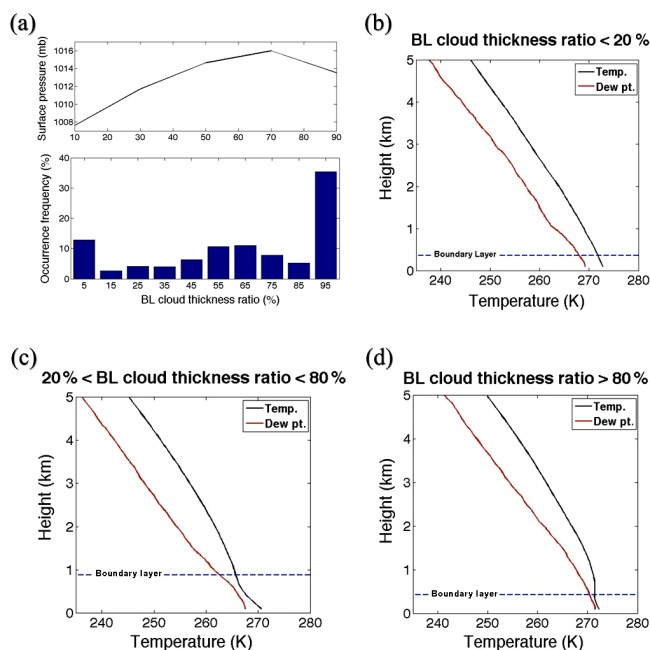
Figure 5. (a) The frequency distribution of BL cloud thickness ratio (bottom panel), and the mean surface pressure for five equally spaced bins of the BL cloud thickness ratio (top panel), and (b) the profiles of mean temperature and dew point temperature observed for cases with BL cloud thickness ratio \leq 20\% , (c) same as (b) but for cases with 20\% < \text{BL cloud thickness ratio} < 80\% , and (d) same as (b) but for cases with BL cloud thickness ratio \geq 80\% .
