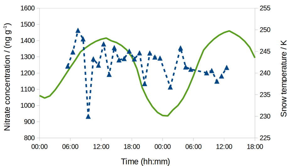
Figure S2. Hourly variations of skin layer nitrate concentration (blue triangles) at DC on 28 and 29 December 2009, and modelled snow surface temperature (solid green line).
