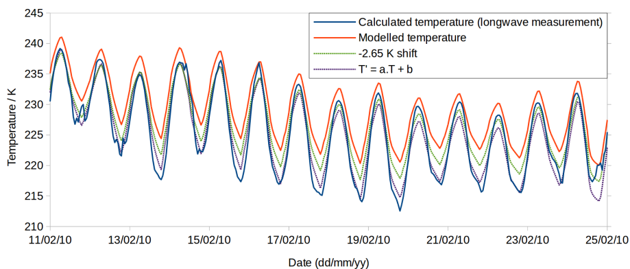
Figure S1. Surface snow temperature deduced from longwave radiation (solid blue line) and modelled temperature used in this study (solid red line). Modelled temperature offset by -2.65 K is plotted in dashed green line. Modelled temperature modified using a linear function to increase its amplitude (see text) is plotted in dashed purple line.
