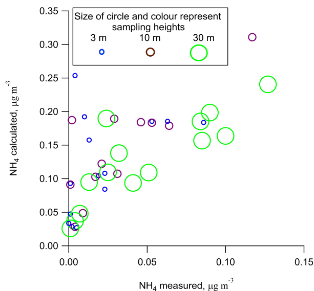
Figure 2. A scatter plot of sulfate neutralisation by ammonium with respect to sampling height.
