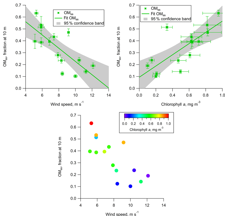
Figure 4. Effect of wind speed and chlorophyll a concentration on the fractional contribution of organic matter (OM ss ): OM ss vs. WS (top left), OM ss vs. chlorophyll a (top right) and OM ss vs. WS coloured by chlorophyll a (bottom). Individual uncertainties of the flux and wind speed are marked with caps, while the grey area denotes 95 % confidence bands of the fitted parameterisation.
