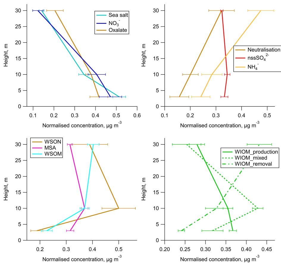
Figure 1. The gradient profiles of chemical species studied: species resembling primary production (top left); inorganic species resembling secondary production (top right); organic secondary species (bottom left); and water-insoluble organic matter split into production, removal and mixed profiles (bottom right).
