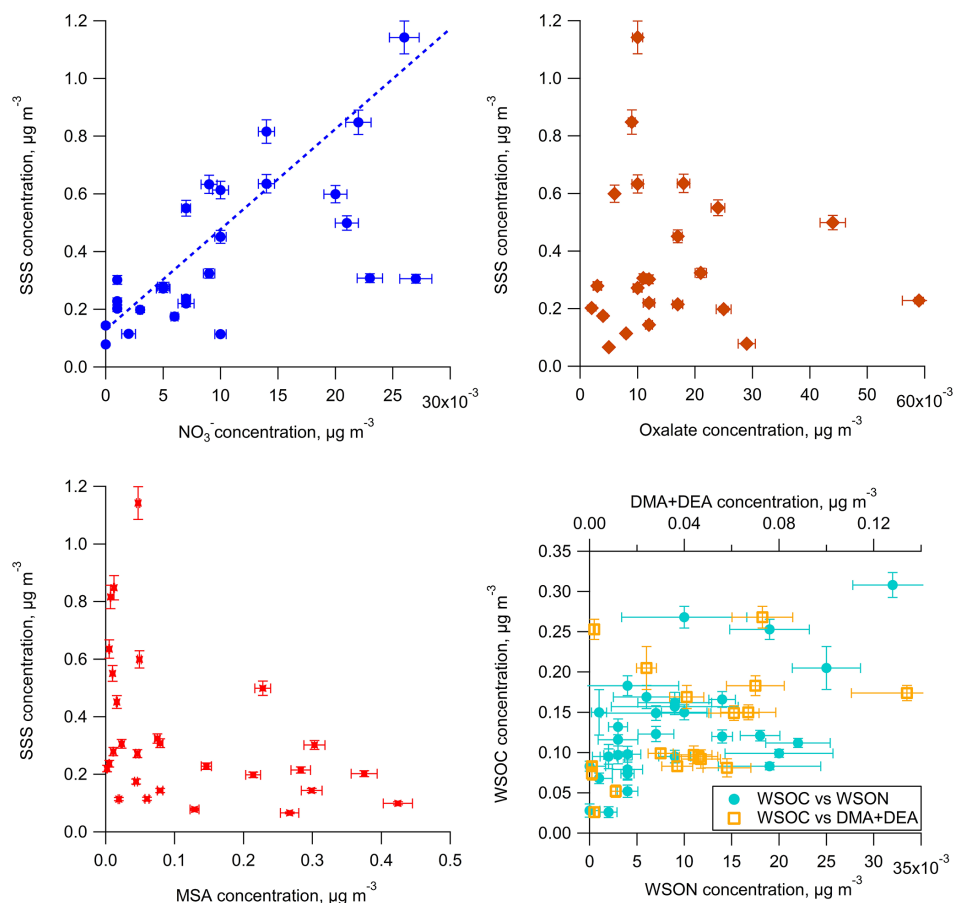
Figure 3. Plots of sea salt and secondary species which resembled primary production concentration pattern: SS vs. NO 3 (top left), SS vs. oxalate (top right), SS vs. MSA (bottom left) and WSOC vs. WSON (also plotted as the sum of dimethylamine and diethylamine) (bottom right). Note that WSOC and WSON concentration are presented as micrograms (µg) of carbon and nitrogen mass, respectively, while all other species are reported in absolute species concentrations.
