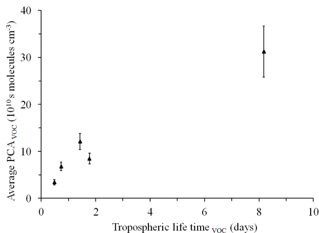
Figure 6. Dependence between average \int[\text{OH}]\text{d}t (photochemical age, PCA) and photochemical lifetime for light aromatic VOC. The average tropospheric lifetime was calculated using the rate constants given in Table 10 and an average tropospheric concentration of 1.16 \times 10^6 OH-radicals \text{cm}^{-3} (Spivakovsky et al., 2000). Vertical error bars are the standard error of the mean.
