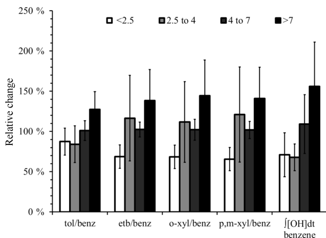
Figure 9. Relative change of VOC concentration ratios and \int[\text{OH}]\text{dt} (PCA) of benzene for different ranges of \int[\text{OH}]\text{dt} (in units of 10^{10} s molecules \text{cm}^{-3} ) derived from the carbon isotope ratio of p,m -xylene. The bars represent the ratio of the mean concentration ratios for the chosen interval of \int[\text{OH}]\text{dt} over the average for all concentration ratios. The error bars are the relative standard errors of the mean. The range of \int[\text{OH}]\text{dt} for the lowest \int[\text{OH}]\text{dt} bin was chosen to include all \int[\text{OH}]\text{dt} , which are not significantly larger than 0. (95 % confidence limit). The other ranges were chosen to include between 8 and 12 data points in each bin.
