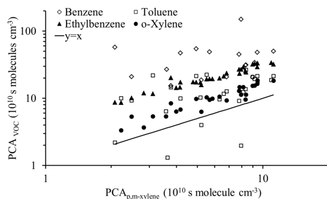
Figure 7. Dependence between the \int[\text{OH}]\text{d}t (PCA) of different VOC and the \int[\text{OH}]\text{d}t (PCA) of p,m -xylene. Only data with \int[\text{OH}]\text{d}t larger than 0 at a 95 % confidence limit are shown.
