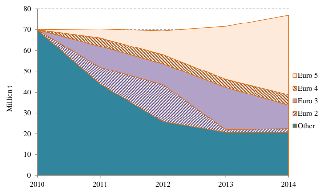
Figure 1. Production of diesel fuel by Euro class in Russia, 2010–2014, in units of Mt. Source: Fedstat (2015c).
