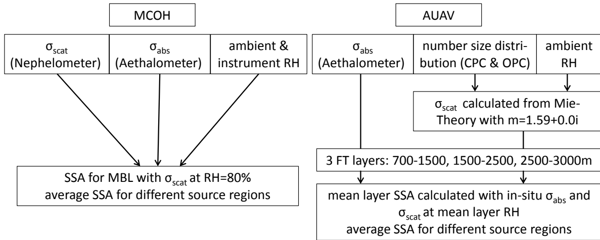
Figure S1: Flow chart describing the derivation of the four layers of the SSA profiles.
