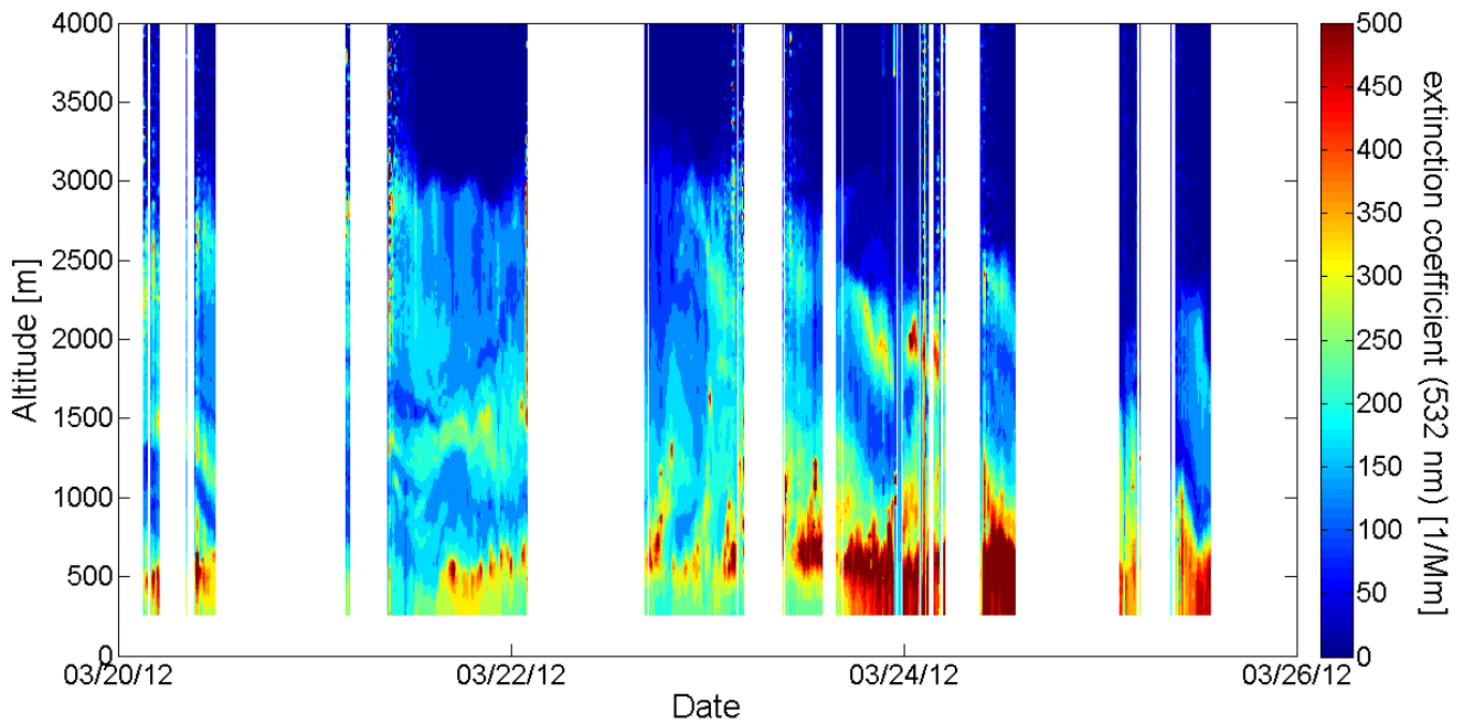
Figure S2: Time series of extinction coefficient profiles determined from MiniMPL measurements from 20 March until 26 March 2012.
