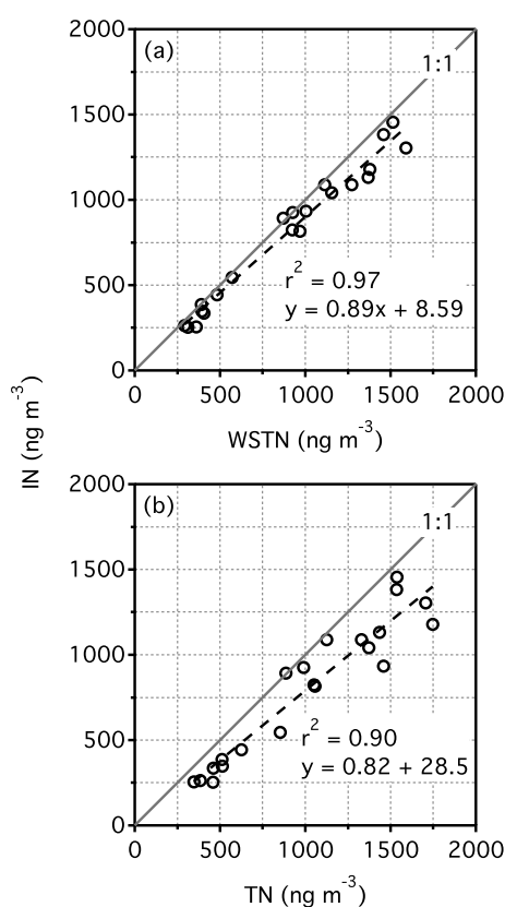
Figure 3. Linear relations of IN (sum of \text{NO}_3^- -N and \text{NH}_4^+ -N) to (a) WSTN and (b) TN.
