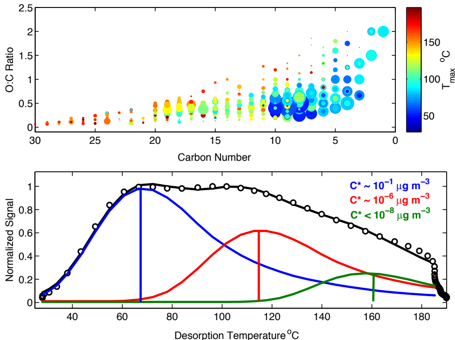
Figure 5. Top: points are plotted sized by the square root of their particle phase desorption signal. Evident is a secondary mode in abundance space between #C 15–20. Each compound is colored by the temperature of maximum desorption signal, which is related to a compound’s enthalpy of sublimation (saturation vapor pressure) as shown previously (Lopez-Hilfiker et al., 2014). Bottom: a sum thermogram, i.e. the entire mass spectral signal at each measurement time (using selection criteria detailed in the text), is summed and plotted vs. desorption temperature. Clearly SOA from \alpha -pinene ozonolysis exhibits multiple modes. The first mode is consistent with monoterpene derived diacids, whereas the secondary modes which arise at temperatures > 100^\circ\text{C} have effective vapor pressures at least 4 orders of magnitude lower than common monoterpene oxidation products.
