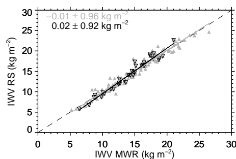
Figure 4. Comparison between IWV from MWR and RS during HOPE. Grey and black triangles indicate all weather conditions and only clear sky conditions, respectively. The solid lines notify the according regression lines. The numbers in the upper left corners denote the bias and the standard deviation, respectively.
