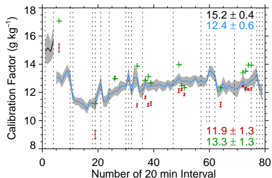
Figure 5. Calibration factor of Polly XT using the IWV method as function of time given in number of 20 min interval. The black and the blue solid lines indicate the calibration factor before and after the major rearrangement of the optical setup on 15 April 2013, 10:06 UTC, respectively. The grey areas denote the standard deviation during each 20 min interval. The numbers represent the according means and standard deviations over the time. The grey dotted lines demonstrate rearrangements on Polly XT especially adjustments of the overlap or cleanups of the quartz plate in the roof of the Polly XT cabinet or they indicate leaps in the time of more than 4 h. The calibration factors of the regression and the profile method are indicated by red points with error bars and green plus signs, respectively.
