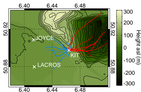
Figure 1. Map of the area around Jülich with westward (blue) and eastward (red) RS trajectories. The darker area in the east indicates the open-cast mining and the brighter area in the north indicates a hill named Sophienhöhe.
