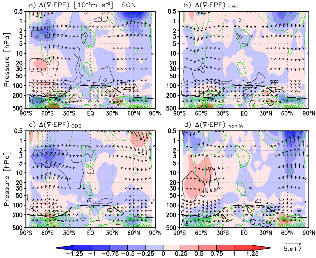
Fig. S1. Latitude-height section of the changes of the Eliassen-Palm flux vectors (in \text{kg s}^{-2} ) and the Eliassen-Palm flux (EPF) divergence (in 10^{-5} \text{ m s}^{-2} ) between 1960 and 2000 for the SON mean (a) and the changes due to GHGs (b) and ODSs (c) as well as the nonlinear contribution (d). Black arrows show the change of the EPF vectors; red/blue shading means positive/negative changes of the EPF divergence. The black contour lines indicate statistically significant changes of the EPF divergence on the 95% confidence level. The green contour lines show the climatology of the EPF divergence for the 1960 reference simulation (R1960). Here, the nomenclature is as follows: A negative EPF divergence is named convergence, while a positive EPF divergence is named divergence. The bold dashed line represents the mean tropopause location of the R1960 simulation for the SON mean.
