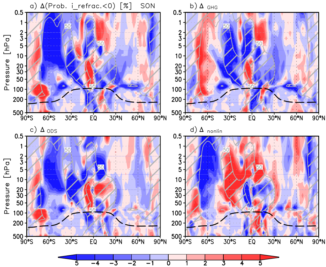
Fig. S2. Same as Figure S1, but for the change in the probability of a negative refractive index. Gray hatching denotes the region where the probability of a negative refractive index is equal or greater than 50% in the R1960 simulation for the SON mean. A negative refractive index means that stationary planetary waves can not propagate and thus a reduced/increased probability of a negative index means that the atmosphere is more/less permeable for waves.
