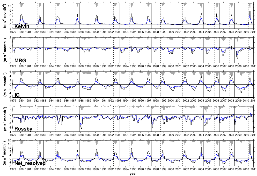
Figure S2. The same as in Fig. 3 except for the forcing averaged over 10^\circ \text{ N} - 10^\circ \text{ S} .
