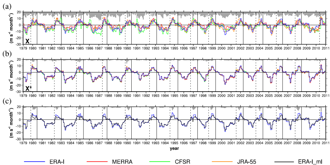
Figure S3. The same as in Fig. 6 except for the forcing averaged over 10^\circ \text{ N} - 10^\circ \text{ S} .
