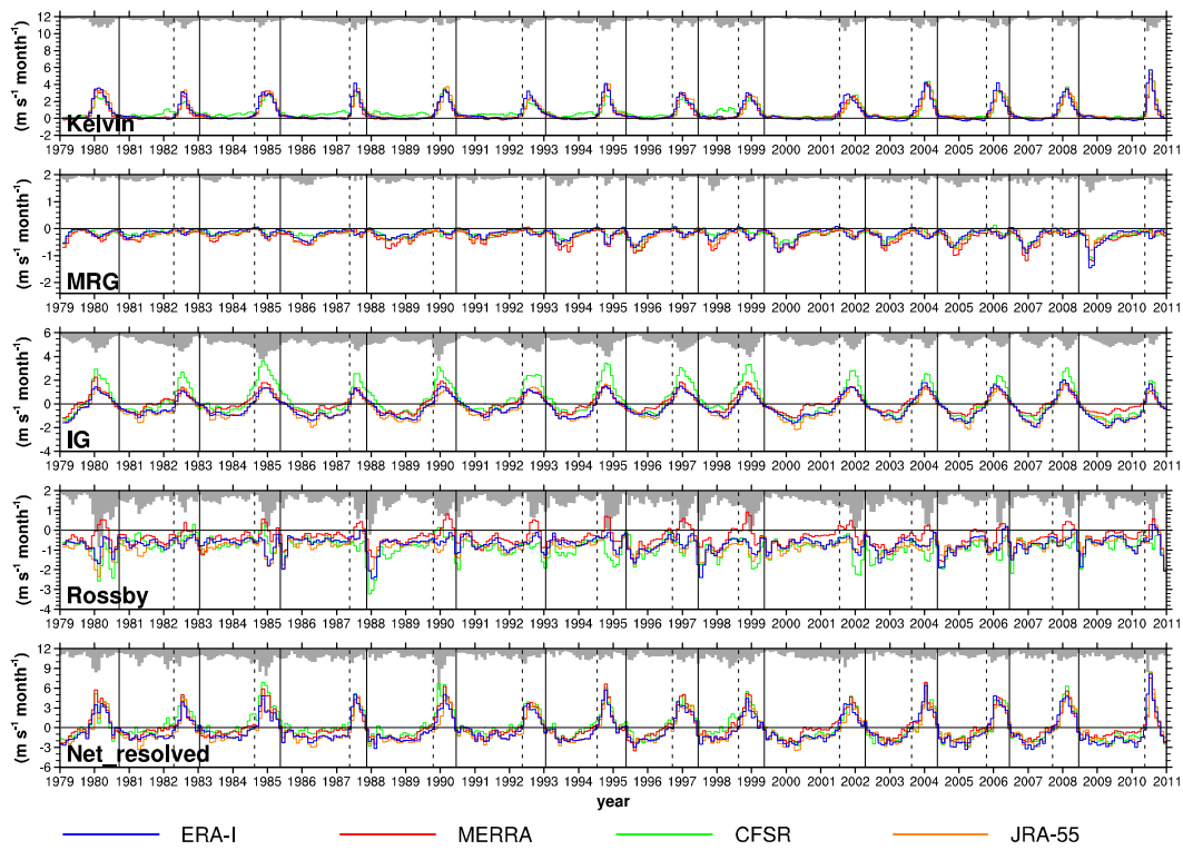
Figure S1. The same as in Fig. 2 except for the forcing averaged over 10^\circ \text{ N} - 10^\circ \text{ S} .
