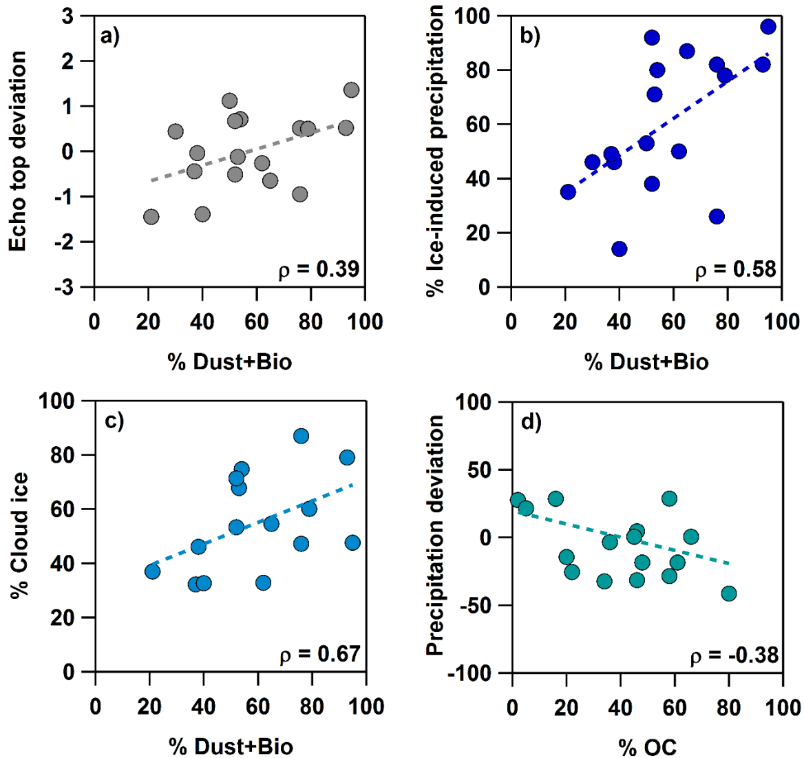
Figure S1. Correlation plots of a) echo top height deviation (km) versus % Dust+Bio, b) % ice-induced precipitation versus % Dust+Bio, c) % cloud ice versus % Dust+Bio, and d) precipitation deviation (mm) versus % OC residues (pollution plus biomass burning). Also shown are the Spearman's correlation coefficients for each correlation.
