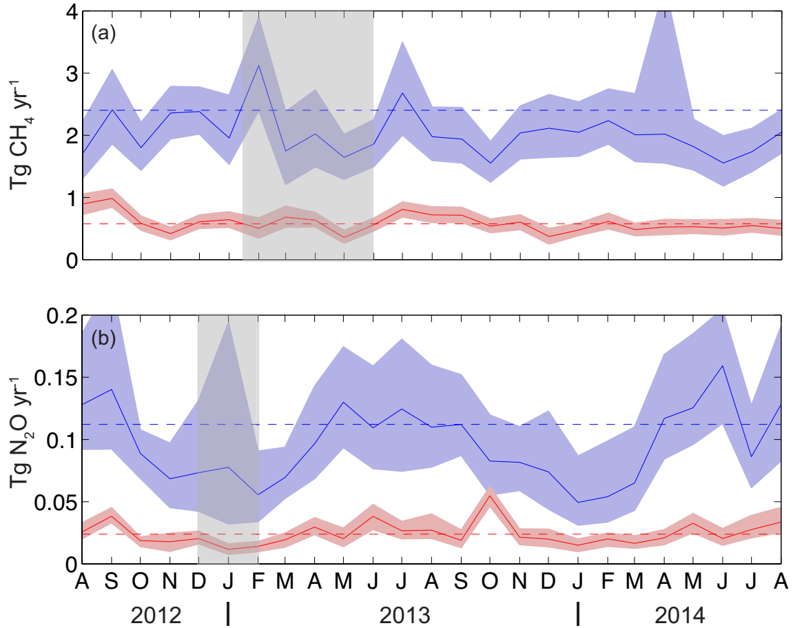
Figure 18: (a) Total national CH 4 and N 2 O emissions for the UK (blue, solid) and Ireland (red, solid) in Tg yr -1 . Prior (anthropogenic only) emissions for each country are shown in the dashed lines. Shading corresponds to the 5th to 95th percentile range.
