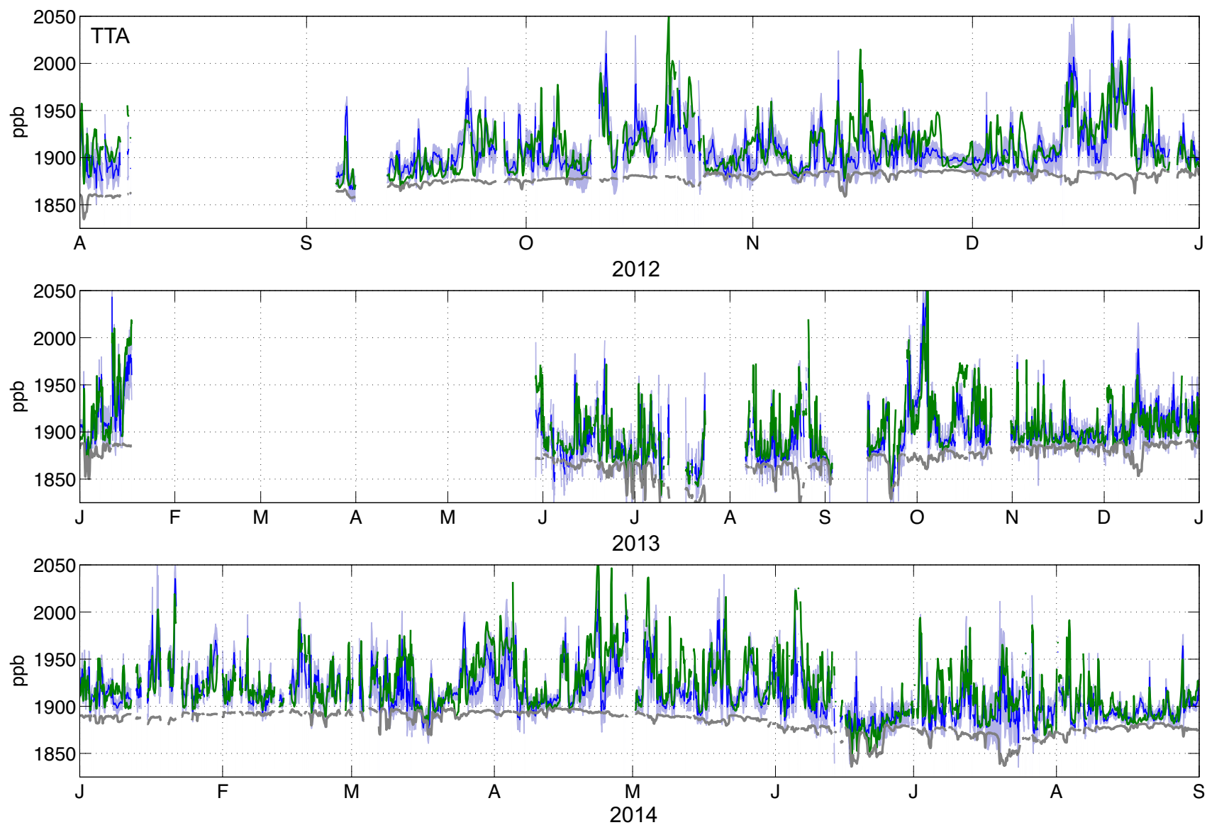
Figure 8: Simulated prior CH 4 mole fractions from TTA by year (green), observations (blue) and derived baseline (grey). Shading indicates the posterior 5th to 95th percentile model errors plus measurement uncertainties.
