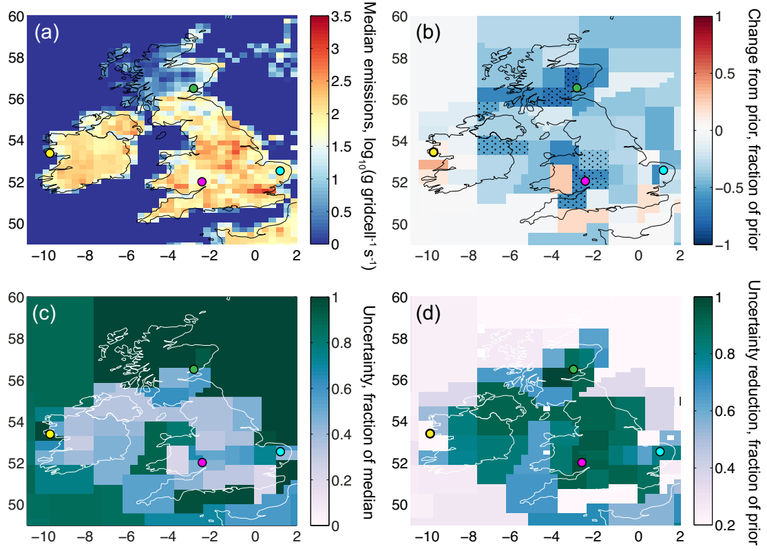
Figure 19: Results derived for the CH 4 sensitivity study in which the prior assumed anthropogenic emissions only. (a) Median posterior CH 4 emissions shown on a logarithmic scale. (b) Fractional difference of the median posterior emissions from the prior. (c) Fractional posterior emissions uncertainty, which corresponds to the difference between the 5th and 95th percentiles, relative to the median. Colored circles show the measurement stations (d) Uncertainty reduction from the prior, relative to the prior (MHD, yellow; RGL, magenta; TAC, cyan; TTA, green).
