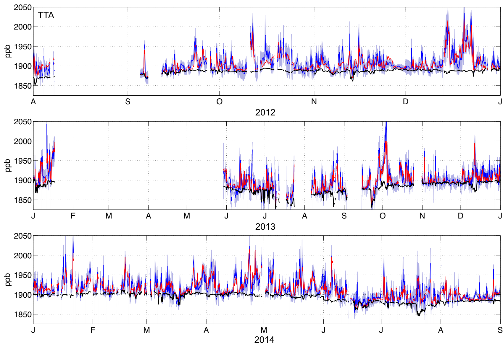
Figure 7: Simulated posterior \text{CH}_4 mole fractions from TTA by year (red), observations (blue) and derived baseline (black). Shading indicates the posterior 5th to 95th percentile model errors plus measurement uncertainties.
