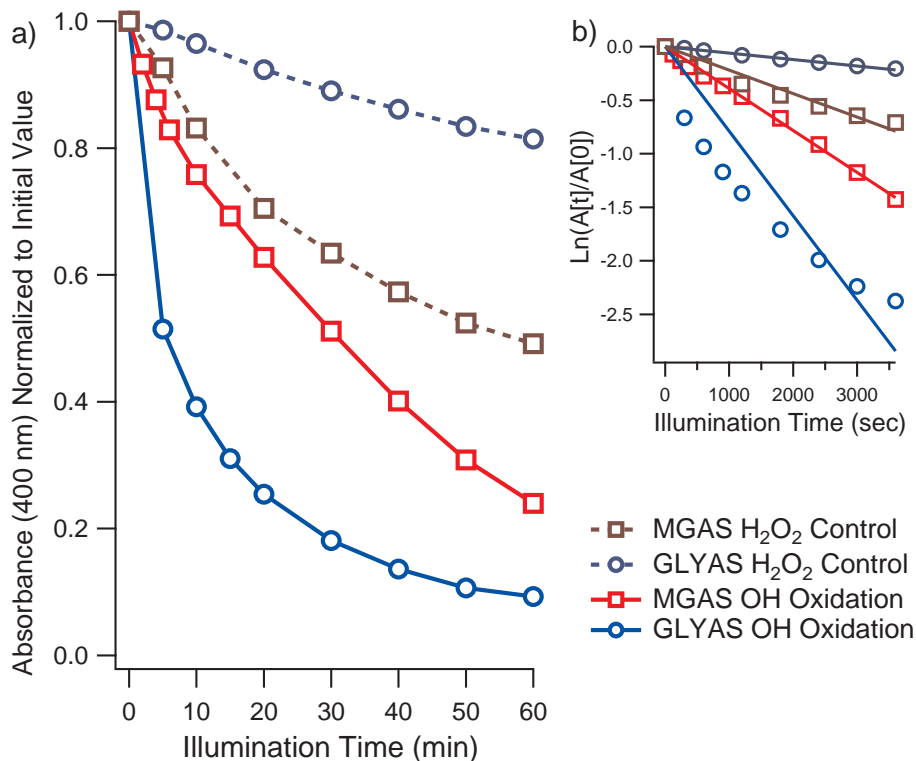
Figure 4. Time profiles of absorbance at 400 nm during OH oxidation (solid lines) and H 2 O 2 control (dashed lines) experiments. Results for both the GLYAS (blue traces) and the MGAS (red traces) solutions are shown. The decay profiles of absorbance at 400 nm normalized to the initial value at t = 0 are shown in (a), while their corresponding 1st order decay plots are shown in (b).
