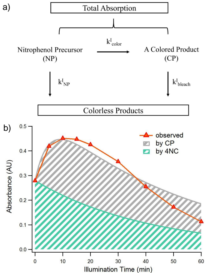
Figure 9. A schematic illustration of the simple kinetic model (a) and one example of 4NC photooxidation (b) . The shaded areas in (b) are the contributions from a newly formed colored product (CP) and the decaying 4NC, respectively. The red line follows data from an experiment.
