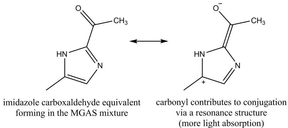
Figure 5. Proposed explanation for the difference in the major bleaching processes of the GLYAS and the MGAS solutions.
