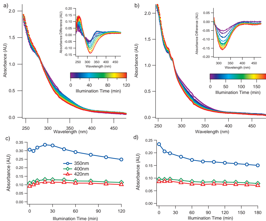
Figure 10. Direct photolysis of the WSOC from biofuel combustion samples. The spectral evolution of the kaoliang and the cotton samples is shown in (a) and (b), respectively. The color code indicates illumination time, while the insets show the absorbance change compared to the initial condition. The time profiles of absorbance at three different wavelengths for the same samples are shown in (c) and (d), respectively.
