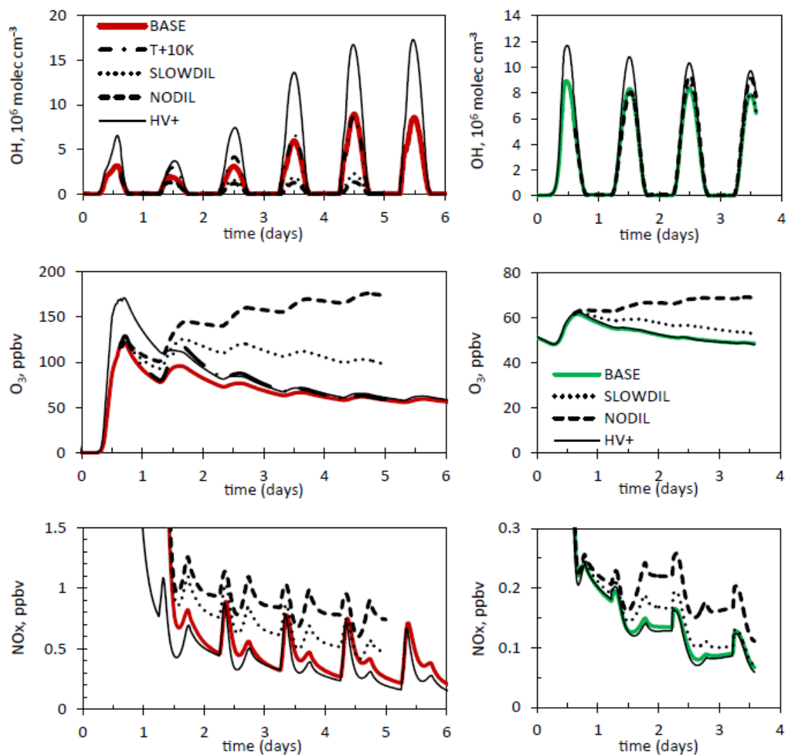
2 3 Figure S1. Timeseries of major oxidants. Left panels show the urban scenario, right panels show the 4 forest scenario. All panels show the reference case and sensitivity cases SLOWDIL, NODIL and HV+. 5 Left panels also show case T+10K.
