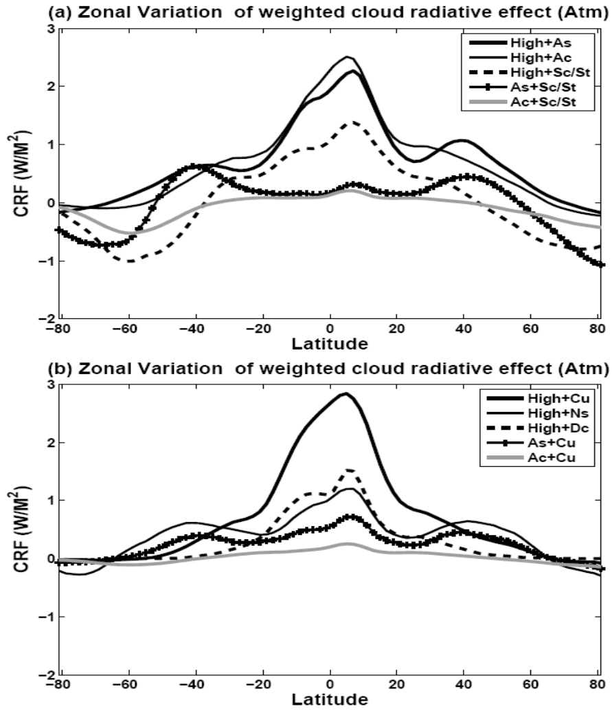
Fig. S1: Same with Figure 5, but in the atmosphere during the daytime.
