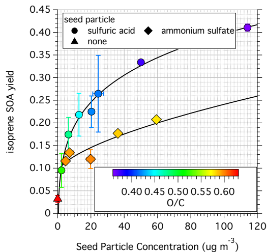
Figure 6. Yields of isoprene SOA produced in the PAM reactor at an OH exposure of 7.8 \times 10^{11} molec \text{cm}^{-3} s as a function of seed particle concentration using ammonium sulfate and sulfuric acid seeds. Error bars indicate \pm 1\sigma uncertainty in binned measurements. Lines are power law fits to guide the eye.
