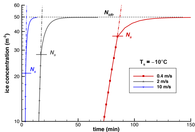
Figure 1. Time evolution of ice particle concentration in a parcel of air undergoing lifting at three different updraft velocities. Cloud base is at 700 mb and +2°C. Lifting stops at -10^{\circ}\text{C} and the parcel remains at that level. The TDFR model is initialized with an INP concentration given by Eq. (3). The horizontal line segments at N_s indicate the ice concentrations when the lifting stops. Note that the greater the updraft velocity is, the lower the value of N_s is. N_{\text{tdfr}} is the asymptotical value of ice concentration while the parcel is at -10^{\circ}\text{C} .
