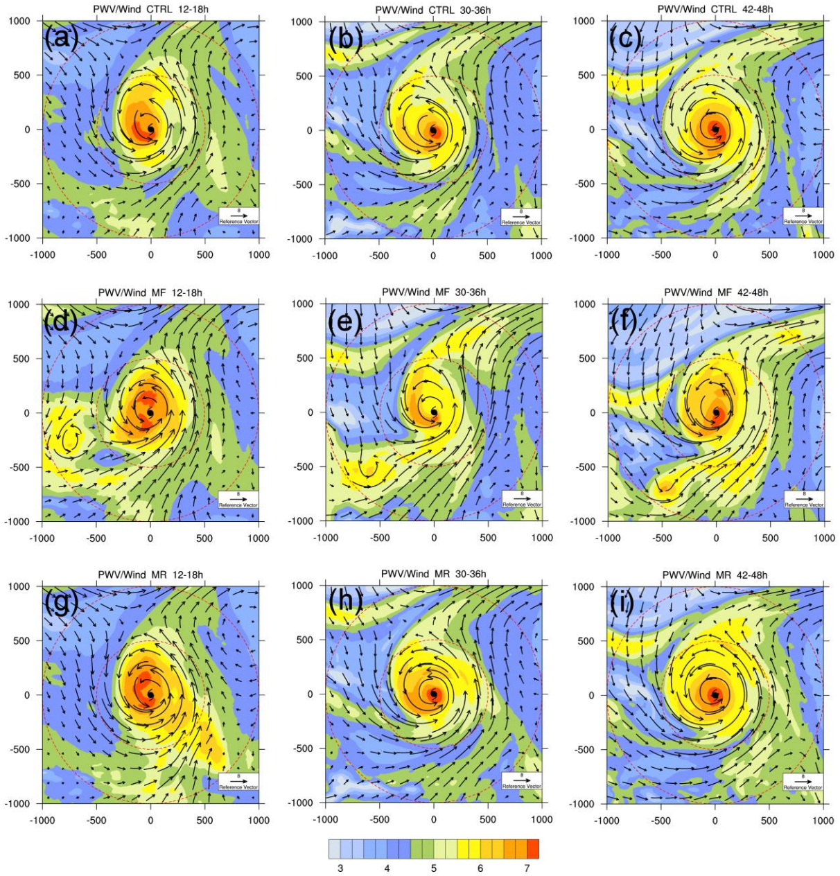
Supplementary Figure 1. Mean wind vector ( \text{m s}^{-1} ) below 5 km and column-integrated PWV (cm) (shading) for CTRL (upper panel), MF (middle panel) and MR (lower panel) at (left panel) 12-18 h; (center panel) 30-36 h; (right panel) 42-48h.
