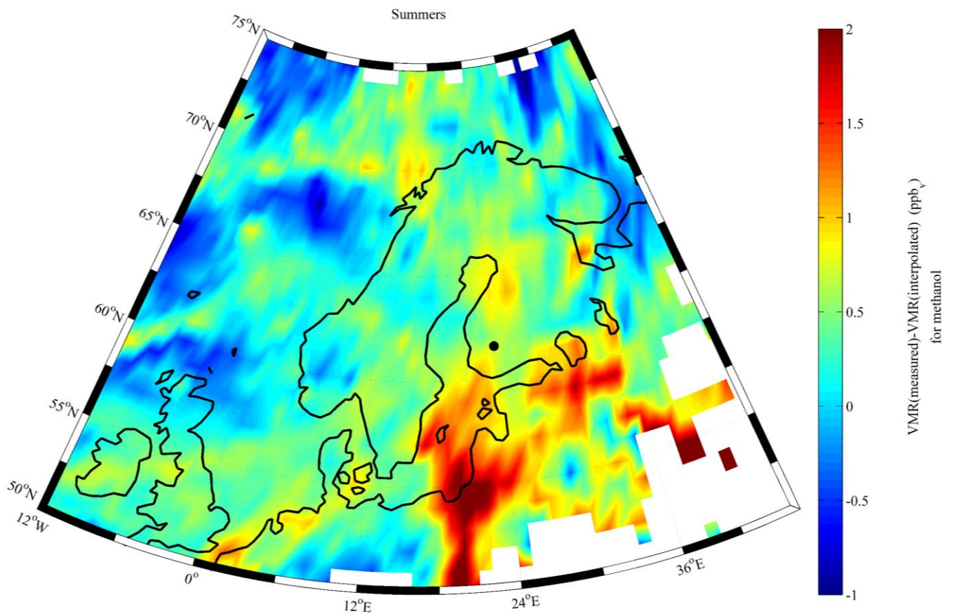
Figure S1. Differential source field for methanol during all summers. Data from forest fire episodes were excluded.
