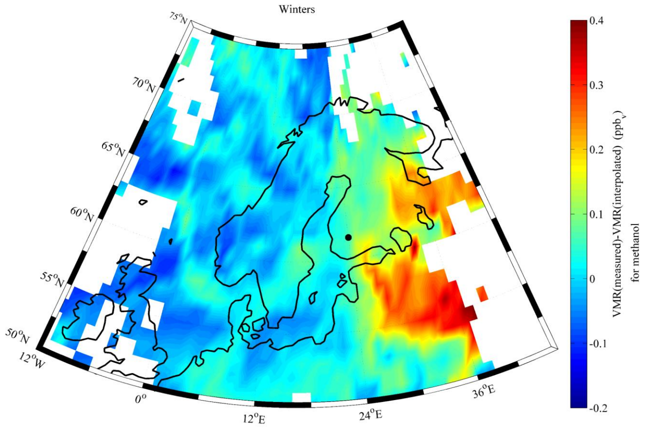
Figure S2. Differential source field for methanol during two winters (2006-2007 and 2008-2009).
