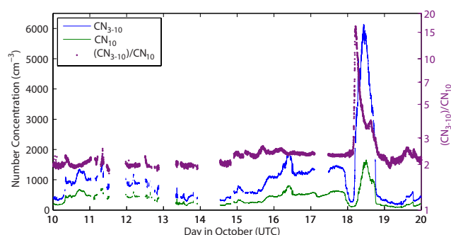
Figure 2. Time series of aerosol parameters for a 10-day subset of the 2012 SIPEXII voyage. Aerosol parameters include calibrated number concentrations of \text{CN}_{3-10} (blue), \text{CN}_{10} (green) and the ratio \text{CN}_{3-10}/\text{CN}_{10} (red). The ratio has been shown previously (Warren and Seinfeld, 1985) to be a good indicator of new particle production when limited measurements are available.
