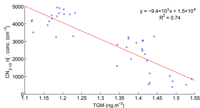
Figure 7. A negative linear correlation is found when \text{CN}_{3-10} was time lagged by 2 h relative to TGM, suggesting involvement of Hg in the nucleation chemistry. Data used show a 5 h period, starting 18 October 02:00 for TGM and 04:00 for CN data. The data gap surrounding TGM concentrations of 1.3 \text{ ng m}^{-3} is a result of routine calibrations, which coincided with the period of interest, and resulted in a 90 min data-gap.
