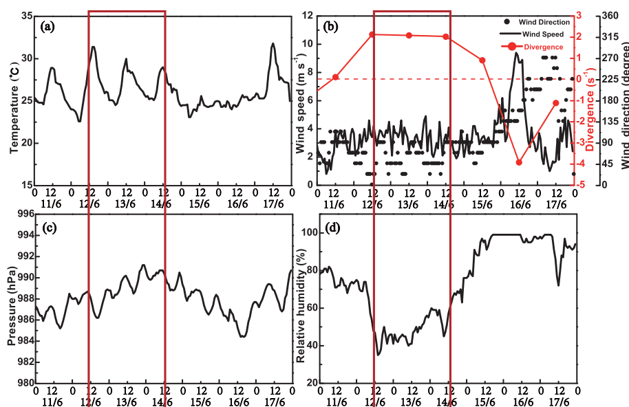
Figure 4. Time series of (a) surface air temperature (b) wind speed, direction and divergence, (c) air pressure and (d) relative humidity observed in the observatory of Xiamen from 11 to 17 June 2014 with the red rectangular columns marking the period of surface O_3 event. The red curve in panel (b) is a daily variation in divergences at 1000 hPa over XQR, calculated with NCEP-FNL data.
