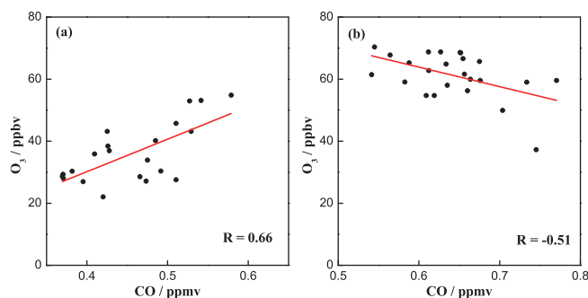
Figure 6. Correlations between measured surface CO and \text{O}_3 over two periods respectively (a) from 12:00 11 June to 12:00 12 June and (b) from 12:00 13 June to 12:00 14 June 2014, passing the significant level of 0.005. Red lines are the linear fittings.
