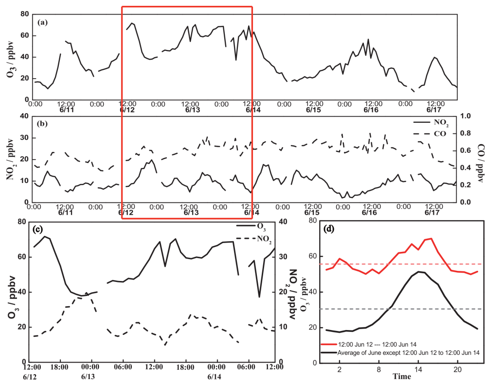
Figure 3. Hourly variations in the eight-site averaged surface concentrations of (a) \text{O}_3 , (b) \text{NO}_2 during 11–17 June with the red rectangular column marking the period of surface \text{O}_3 event and (c) \text{O}_3 and \text{NO}_2 for the surface \text{O}_3 event over XQR, as well as (d) diurnal changes of surface \text{O}_3 from 12:00 12 June to 12:00 14 June (red curve) and in June excluding 12–14 June 2014 (black curve) with two dotted lines indicating the daily averaged \text{O}_3 concentrations for two diurnal curves.
