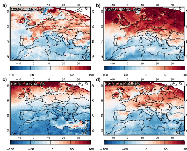
Figure 7. The same as Fig. 1 but for RegCM4 and CM SAF COT.
