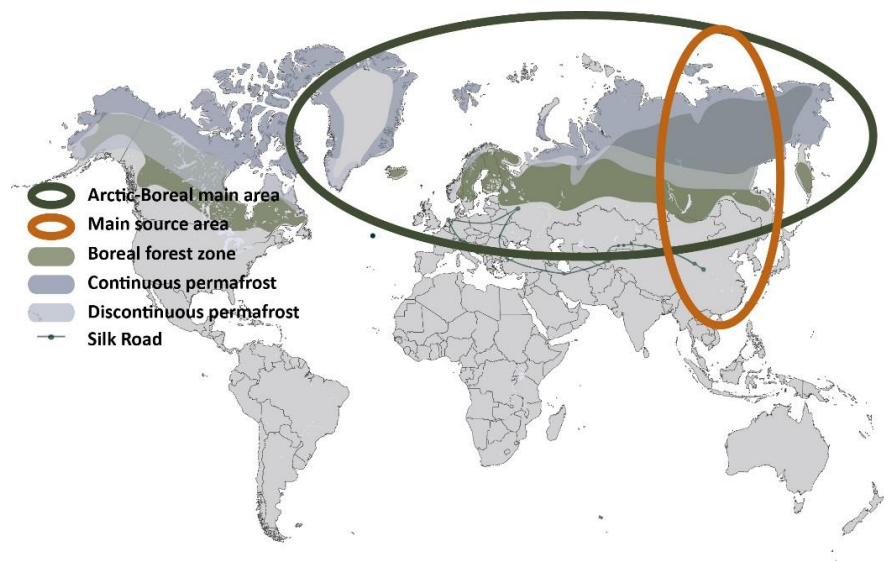
Figure 2. Northern Pan-Eurasian geographical region encompasses both permafrost and boreal zones.
