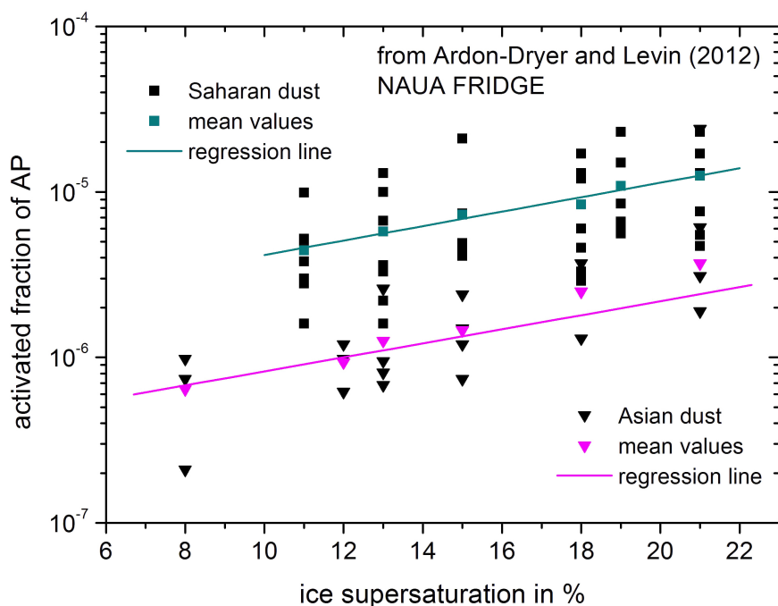
Figure 5. Activated fraction of particles in the deposition freezing mode as a function of ice supersaturation for Saharan and Asian dust. Data from K. Ardon-Dryer and Z. Levin (personal communication, 2012).
