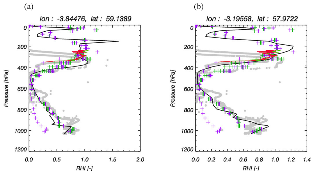
Figure 8. A comparison between the retrievals, dropsonde measurements, in situ measurements and NWP model predictions of RH_i plotted against the pressure (hPa) for two different locations. (a) The pixel located at longitude -3.84 and latitude 59.14^\circ and (b) the pixel located at longitude -3.20 and latitude 57.97^\circ . In (a) and (b), the retrievals are represented by the purple and green plus signs, dropsonde measurements are the solid grey line and filled grey circles, the General Eastern hygrometer is the solid green line, and the FWVS hygrometer is the solid red line.
