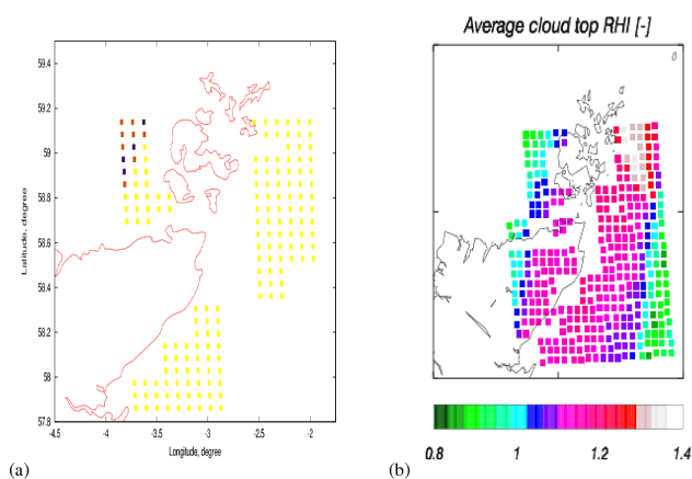
Figure 11. Associating the PARASOL estimations of shape of the scattering phase function at each pixel to the NWP-model-predicted field of RH_i . (a) The estimated shape of the scattering phase function; the yellow squares are as previously defined in Fig. 9. The brown squares represent those PARASOL pixels where no phase function model could be assigned, and the blue squares represent those pixels where phase function models assuming distortion values of between 0 and 0.25 could be assigned. (b) The NWP-model-predicted cloud-top RH_i field, where the colour bar indicates the range in predicted RH_i .
