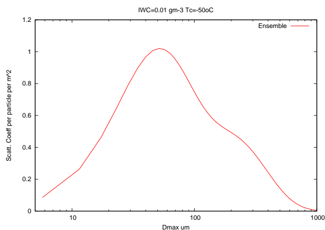
Figure 5. The scattering coefficient per particle ( \text{m}^{-2} ) as a function of ice crystal maximum dimension, D_{\text{max}} . The PSD was generated assuming IWC and in-cloud temperature values of 0.01 \text{ gm}^{-3} and -50 \text{ }^{\circ}\text{C} , respectively.
