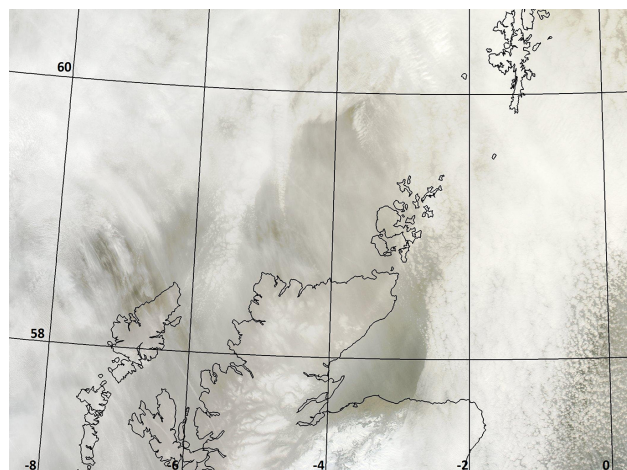
Figure 1. A high-resolution composite MODIS image of the semi-transparent cirrus case that occurred on 25 January 2010 located over north-east Scotland. The latitude and longitude grid is superimposed on the image showing latitude 58 to 60^\circ (left side) and longitude -8 to 0^\circ (bottom). The composite image was formed by combining the MODIS red, green and blue channels to obtain the closest “true” colour image. The image is from the NERC Satellite Receiving Station, Dundee University, Scotland ( http://www.sat.dundee.ac.uk/ ).
