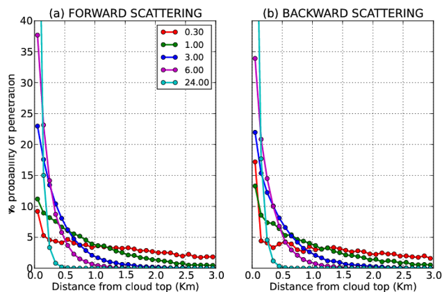
Figure 12. The percent (%) probability of the penetration depth of solar radiation at 0.865\ \mu\text{m} as a function of distance from the cloud top (km), and cloud optical depth for (a) forward-scattered and (b) backward-scattered solar radiation in the principal plane, respectively. The percent probability of penetration is defined as the last position (distance from the cloud top) of the photon before leaving the cloud to reach the sensor. The cloud optical depth colour scale is defined by the key shown on the upper right-hand side of (a).
