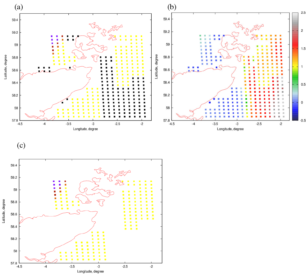
Figure 9. The PARASOL estimates of ensemble model randomisations (based on minimised RMSE) and retrievals of optical thickness as a function of latitude and longitude. (a) The estimated ice crystal randomisation, where the indeterminate results are shown by the black squares, the most randomised phase functions (distortion = 0.4 with spherical air bubble inclusions) by the yellow squares, and the pristine phase functions (distortion = 0) by the purple squares; dark- and light-brown squares represent the slightly distorted (distortion = 0.15) and moderately distorted (distortion = 0.25) phase functions, respectively. (b) The PARASOL-retrieved averaged optical thickness, averaged over all scattering angles, where the decadal logarithm of the retrieved optical thickness is shown by the colour bar on the right-hand side of the figure. (c) The same as (a) but with the indeterminate results removed.
