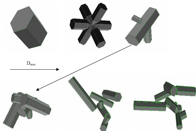
Figure 2. The ensemble model as a function of ice crystal maximum dimension, D_{\max} . The first element of the model is the hexagonal ice column of aspect ratio unity (first top left), followed by the 6-branched bullet rosette (top centre), the 3-monomer hexagonal ice aggregate (top right), 5-monomer ice aggregate (first bottom left), 8-monomer ice aggregate (bottom centre) and the 10-monomer ice aggregate (bottom right).
