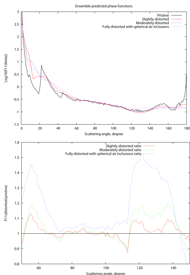
Figure 4. (a) The decadal logarithm of the ensemble model normalised scattering phase function as a function of scattering angle assuming a variety of distortions. The model cases shown are the pristine (black), slightly distorted (red), moderately distorted (dashed blue) and fully distorted with spherical air bubble inclusions (dotted purple). (b) The ratio between the distorted and pristine ensemble model phase functions as a function of scattering angle. Shown here are slight distortion (red), moderate distortion (dotted green) and full with spherical air bubble inclusions (dotted blue). The key is shown in each of the figures.
