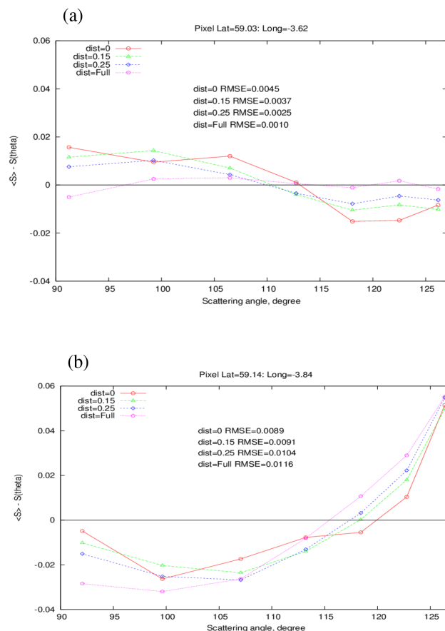
Figure 10. Differences between the directionally averaged ( \langle S \rangle ) and directional ( S(\theta) ) spherical albedos as a function of scattering angle at two pixel locations. (a) The spherical albedo differences for the pixel located at 59.03° and longitude -3.62°, assuming the pristine ensemble model (dist = 0) (open red circles), the slightly distorted model (dist = 0.15) (open green triangles), the moderately distorted model (dist = 0.25) (open blue diamonds), and the fully randomised model (dist = 0.4 with spherical air bubble inclusions) (open purple pentagons). (b) The same as (a) but for the pixel located at latitude 59.14° and longitude -3.84°. The zero difference line is shown by the solid bold line, and the RMSE values calculated for each of the models are shown in each of the figures.
