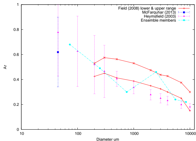
Figure 3. The ensemble model area ratio, A_r , as a function of ice crystal diameter or D_{\max} . The key is shown on the upper right-hand side of the figure. The members of the ensemble model are represented by the filled cyan circles. The in situ observations are represented by the Field et al. (2008) (red lines), where the plus and cross signs represent the lower and upper range of those observations and those ranges have an uncertainty of \pm 30\% . The blue error bar represents the mean and range of observations taken from McFarquhar et al. (2013) and the purple error bars represent the uncertainty in the observations taken from Heymsfield and Miloshevich (2003).
