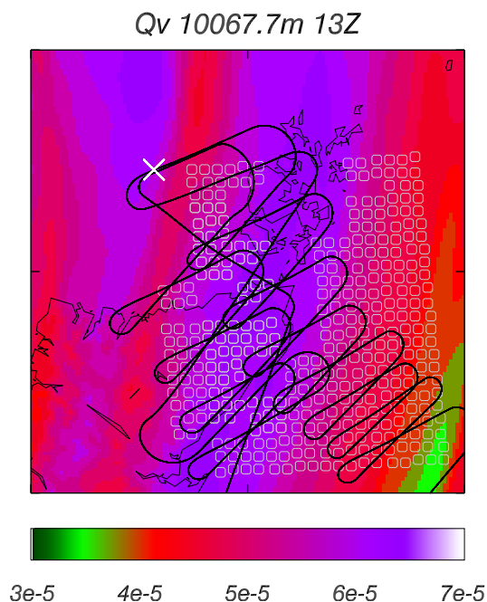
Figure 6. The UKV-model-predicted field of the water vapour mixing ratio ( Q_v ) on 25 January 2010 at 13:00 UTC, between latitudes 57.8 and 59.7^\circ and longitudes -5.3 and -1.8^\circ . The units of Q_v are \text{Kg Kg}^{-1} . The PARASOL pixels are represented by the open circles and the aircraft track is represented by the solid line, and X marks the location where the aircraft was directly above the cloud at about 13:33:00 UTC.
