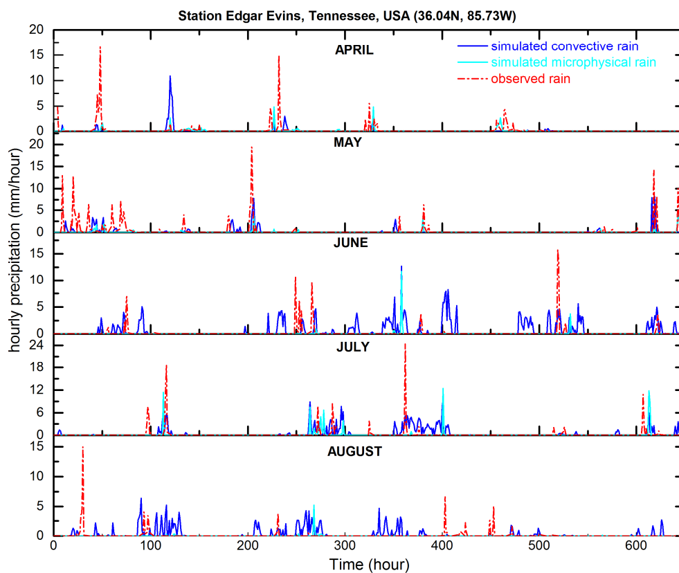
Figure S1. Comparison of simulated hourly convective and non-convective (microphysical) precipitation with the observations for individual months from April to August 2009.
