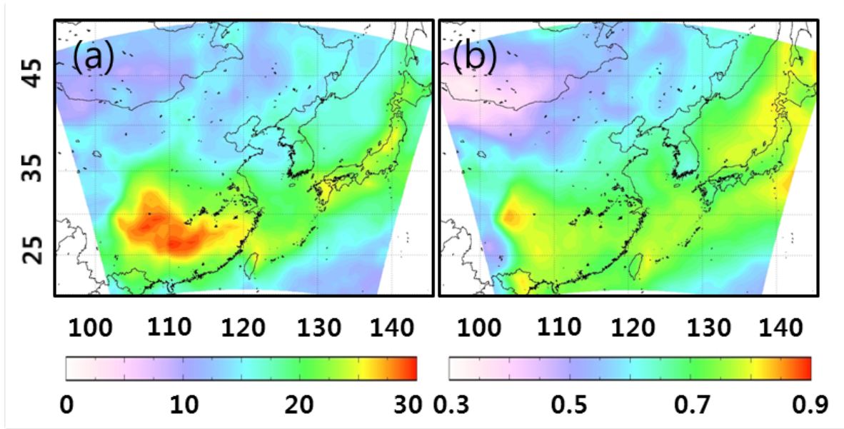
Figure S1. Spatial distributions of (a) cloud optical depth (COD) and (b) cloud fraction obtained from MODIS over East Asia for 2006.
