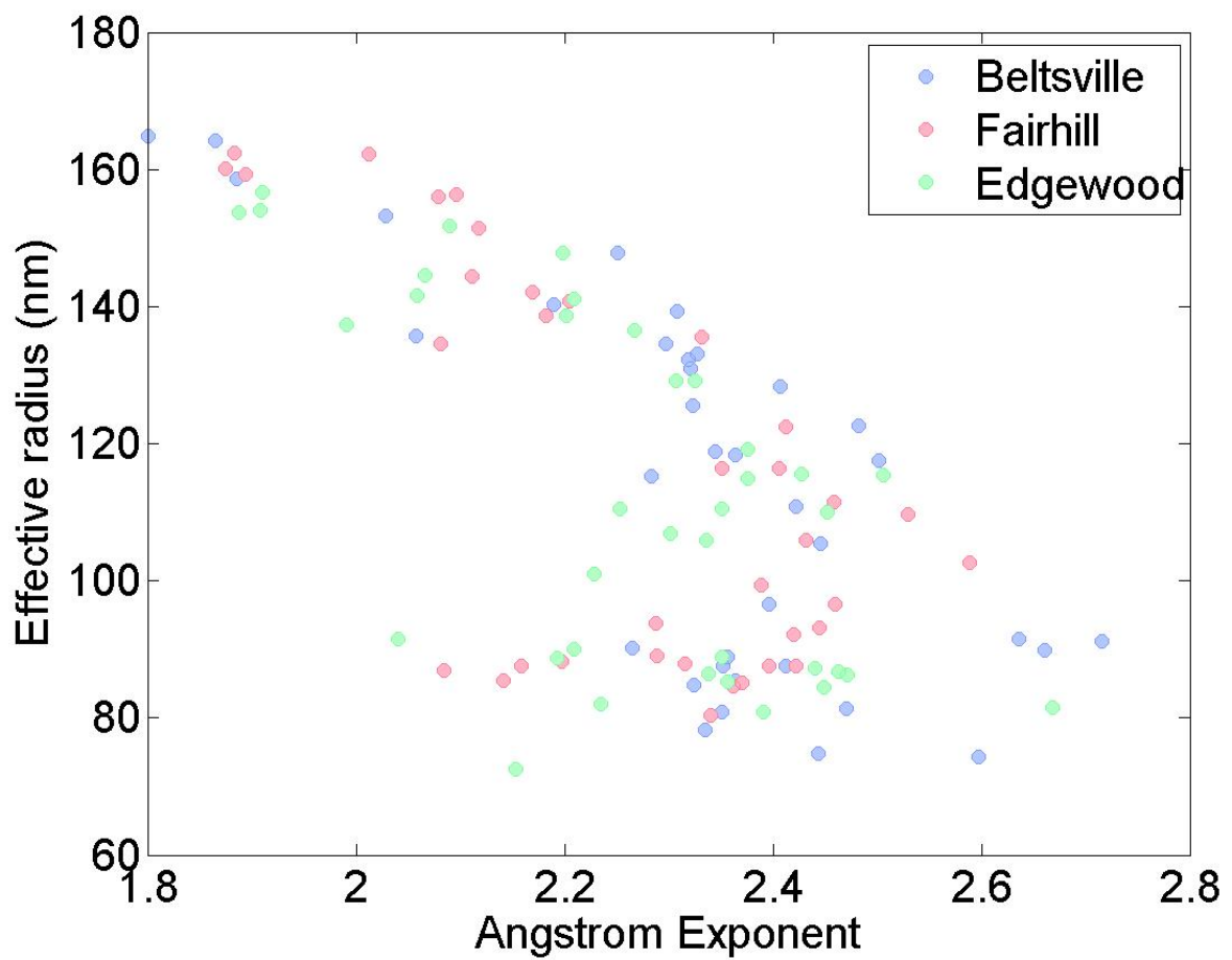
Figure 1 : Effective radius (nm) as a function of the Ångström exponent (450-700nm) measured aboard the P3-B over Beltsville, Fairhill and Edgewood during the entire campaign.
